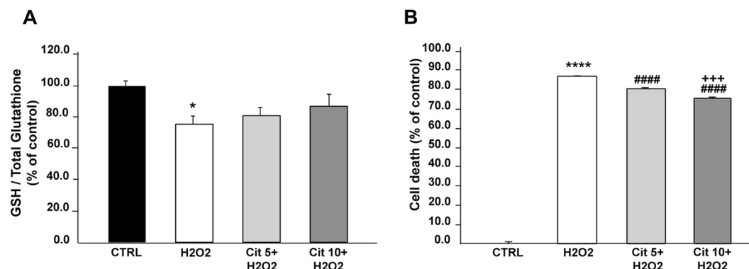
Figure 1. Protective effect of Cit against H 2 O 2 -induced oxidative stress in SH-SY5Y cell line. (A) Cit effect on intracellular oxidative stress (IOS). IOS was assessed by GSH/Total Glutathione ratio and expressed as % of control. GSH/Total glutathione ratio has been assessed in control conditions (CTRL), after oxidative stress induced by H 2 O 2 500 \mu M (H 2 O 2 ), after H 2 O 2 500 \mu M in the presence of Cit 5 mM (Cit 5 + H 2 O 2 ) or Cit 10 mM (Cit 10 + H 2 O 2 ). The significant decrease in GSH/Total glutathione ratio is shown by * (* p < 0.03). (B) Cit effect on H 2 O 2 -induced cell death. Cell death has been assessed in control condition (CTRL), after treatment with H 2 O 2 500 \mu M (H 2 O 2 ) alone and in the presence of Cit 5 mM (Cit 5 + H 2 O 2 ) or Cit 10 mM (Cit 10 + H 2 O 2 ). The results are expressed as % of control. The significances are designed as followed: *: H 2 O 2 vs CTRL; #: Cit + H 2 O 2 vs H 2 O 2 ; +: Cit10 + H 2 O 2 vs Cit5 + H 2 O 2 . (**** p < 0.0001; #### p < 0.0001; +++ p = 0.0001). Data in A and B are presented as the mean \pm SEM of 4 independent experiments.
