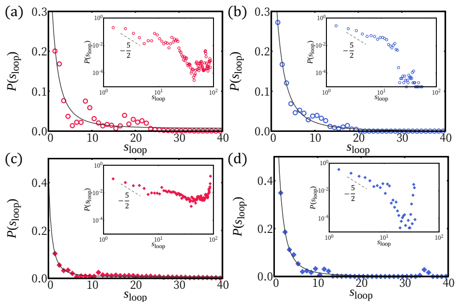
Figure 5. The loop length distributions of H-filament \gamma > 1 (a,b) and \gamma < 1 (c,d) for the two representative values of \epsilon : weak adsorption regime ( \epsilon = 0.1 ) (a,c); and strong adsorption regime ( \epsilon = 1.0 ) (b,d). The envelop of distributions in general follows WLC statistics s^{-5/2} (with an offset \lesssim 1 in s ), which is represented as solid line.
