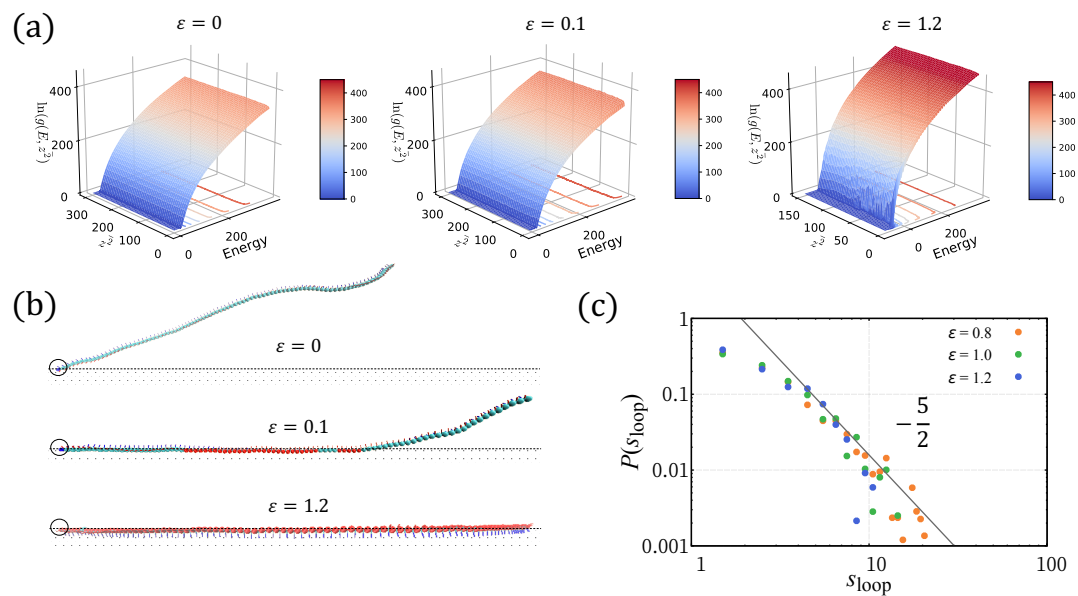
Figure A2. (a) DOS g(E, z^2) of WLCT filament interacting with short range attractive potential. (b) Representative conformation of WLCT at weak ( \epsilon = 0.1 ) and strong ( \epsilon = 1.2 ) adsorption regime. (c) Loop length distribution P(s) . The line represent the scale of adsorption loop length distribution P(s) \propto s^{-5/2} .
