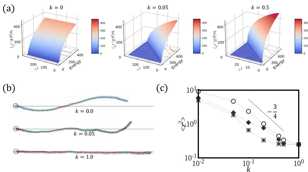
Figure A1. (a) DOS g(E, \bar{z}^2) of WLCT under various strength of harmonic potential V(z) = \frac{1}{2}kz^2 , k = 0, 0.05 (weak confinement) and k = 0.5 (strong confinement). (b) Loops of WLCT at various k . (c) \langle z^2 \rangle of WLCT in harmonic potential confinement in log-log scale for k = 0.05, 0.1, 0.2, 0.4 , and 1.0 from top to bottom. The line is used to guide the eye and represents \langle z^2 \rangle \propto k^{-3/4} .
