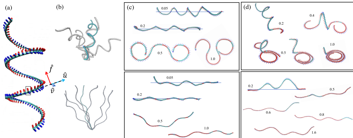
Figure 1. Various shapes of super-Helical filaments. (a) The helical shape of the ground state conformation of H-filaments ( \omega_1 = 0.81\sigma^{-1} , \omega_2 = 0 , and \omega_3 = 0.10\sigma^{-1} ). The local twist and curvature are represented by a set of orthogonal vectors \{\hat{u}, \hat{f}, \hat{v}\} along the filament backbone. \hat{f}, \hat{v} are defined in the material frame orthogonal to the local tangent vector \hat{u} . Top panels in (b–d) show H-filaments with \gamma > 1 , ( \omega_1 = 0.81\sigma^{-1} , \omega_2 = 0 , and \omega_3 = 0.10\sigma^{-1} ), where circular shapes are ground states when squeezed. Bottom panels in (b–d) show H-filaments with \gamma < 1 , ( \omega_1 = 0.09\sigma^{-1} , \omega_2 = 0 , and \omega_3 = 0.19\sigma^{-1} ), where wavy shapes are ground states when squeezed. The localized parts of H-filaments ( |z| < 0.2\sigma ) are shown in red. (b) Bulk conformations subject to thermal fluctuations. (c) Typical conformations of H-filaments confined by harmonic potential V(z) = \frac{1}{2}kz^2 and (d) adsorbed under a localized surface potential U_{ads}(z) = 4\epsilon[(\sigma/z)^{12} - (\sigma/z)^6] . The numbers are the strength of harmonic potential k and the surface potential \epsilon . The figures with horizontal lines indicating the line of z = 0 are side views. The flexural modulus B = 50\sigma k_B T and twist modulus C = B/2 .
