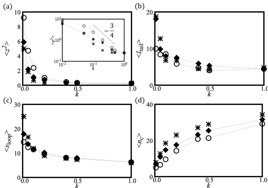
Figure 2. Various measured properties of H-filaments, consisting of N = 90 monomers, confined by a harmonic potential V(z) = \frac{1}{2}kz^2 . One end is anchored at z = 0 . Symbols \circ , filled \circ , and * , respectively, stand for: (i) \gamma > 1 ; (ii) \gamma < 1 ; and WLCT ( \omega_1 = \omega_2 = \omega_3 = 0 ). (a) The height fluctuation \langle z^2 \rangle as the function of the stiffness k of the harmonic potential. The solid line represents analytical calculation in weak fluctuation limit (Equation (11)) for Case (i), \omega_1 = 0.18\sigma^{-1} , and \omega_3 = 0.10\sigma^{-1} . The inset shows mean squared height \langle z^2 \rangle as a function k on log-log scale. The solid line is used to guide the eye for the exponent in relation \langle z^2 \rangle \propto k^{-3/4} expected for the WLC. (b) Average tail length \langle l_{\text{tail}} \rangle ; (c) average loop length \langle s_{\text{loop}} \rangle ; and (d) mean number of confined monomers \langle n_c \rangle .
