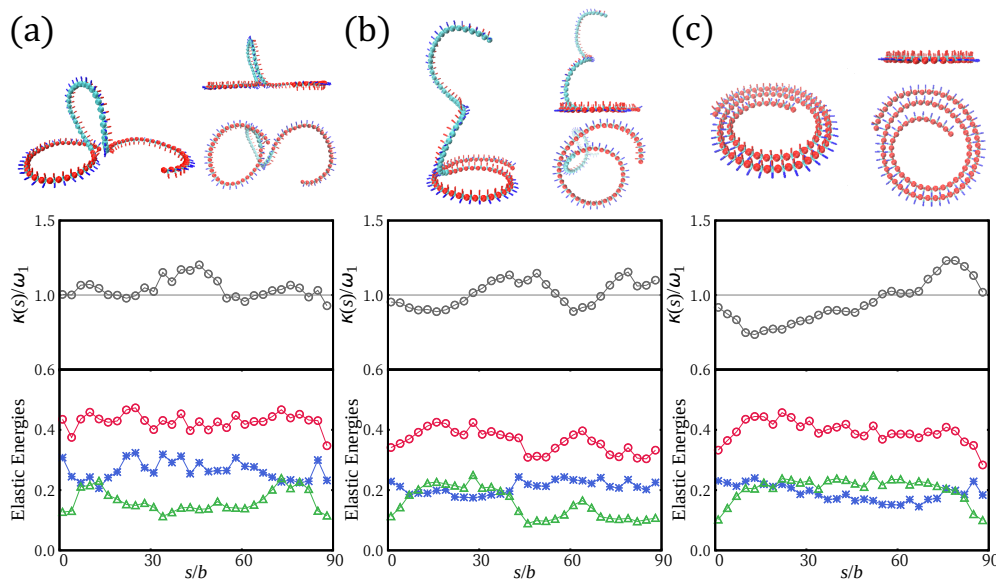
Figure 6. Three representative shapes of adsorbed H-filaments ( \gamma > 1 ) at: (a) \epsilon = 0.4 ; (b) \epsilon = 0.8 ; and (c) \epsilon = 1.6 . The localized parts are shown in red. The middle panels show measured local curvatures \kappa(s) relative to the preferred curvature \omega_1 = 0.181 . Local curvatures \kappa(s) = \sqrt{\Omega_1^2 + \Omega_2^2} ( \circ ) are averaged over several similar conformations along the contour s . Lower panels show twist energy density (green \Delta ), bending energy density (blue * ), and the sum of these two (red \circ ).
