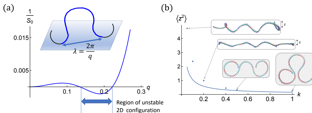
Figure 7. (a) The bare inverse structure factor S_0^{-1}(q) defined in Equation (10) (i.e., k = 0 ) for \omega_1 = 0.18 and \omega_3 = 0.10 . Boundary conditions impose flat circular shapes outside of the section of interest. Note the region of instability indicated by negative S_0^{-1} . The harmonic potential of strength k would shift the inverse structure factor upwards by k , S_k^{-1}(q) = S_0^{-1} + k . Hence, k > 0.005 stabilizes the flat helical chain against small amplitude fluctuations. In practice, larger k is required to ensure the validity of the quadratic expansion. (b) The height fluctuation \langle z^2 \rangle in weak fluctuation limits as a function of the stiffness fk of the harmonic potential for helical filament (i), \omega_1 = 0.18\sigma^{-1} , \omega_3 = 0.10\sigma^{-1} . Analytical calculation following Equation (11) is shown as solid line and the simulation data for filaments with one end anchored are shown in dots together with typical conformations at some k -values. Flat configurations at k = 0.5 and 1.0 are captured from the top view.
