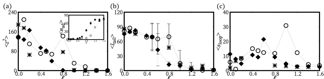
Figure 4. H-filaments adsorbed in a localized surface potential U_{ads} . Various properties are measured for a H-filament of length S = 90\sigma with one of its ends anchored at z = 0 . Symbols \circ and filled \diamond stand for the case of \gamma > 1 and \gamma < 1 , respectively. WLCT case at strong/weak adsorption regimes are represented as *. (a) \langle z^2 \rangle at various strengths of surface potential \epsilon . The inset shows the average number of the adsorbed monomers ( |z| < 0.2 ). (b) Average tail length \langle l_{tail} \rangle ; and (c) average loop length \langle s_{loop} \rangle at various \epsilon .
