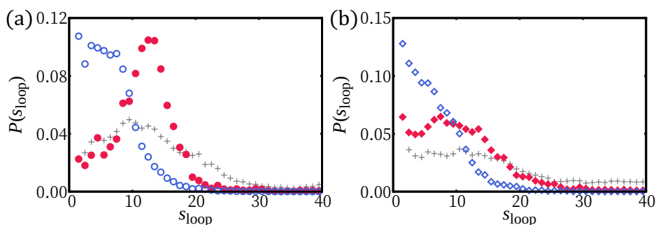
Figure 3. The loop length distributions for: (a) \gamma > 1 ( \circ ); and (b) \gamma < 1 ( \diamond ). Loop length is defined as the segment length that consecutively belongs to |z| > 0.2 . Two representative regimes, weak confinement regime k = 0.05 and strong confinement regime k = 1.0 , are shown by filled and empty symbols, respectively. The loop distribution with k = 0 is shown as gray symbols (+) for comparison. For \gamma > 1 , the loop length making half of the 3D helical period is most prevalent at weak confinement. Smaller loops are equally common for \gamma < 1 , where the H-filament is more confined (see Figure 1a). Strongly confined segments show almost flat distributions for \gamma > 1 and two sub-populations for \gamma < 1 .
