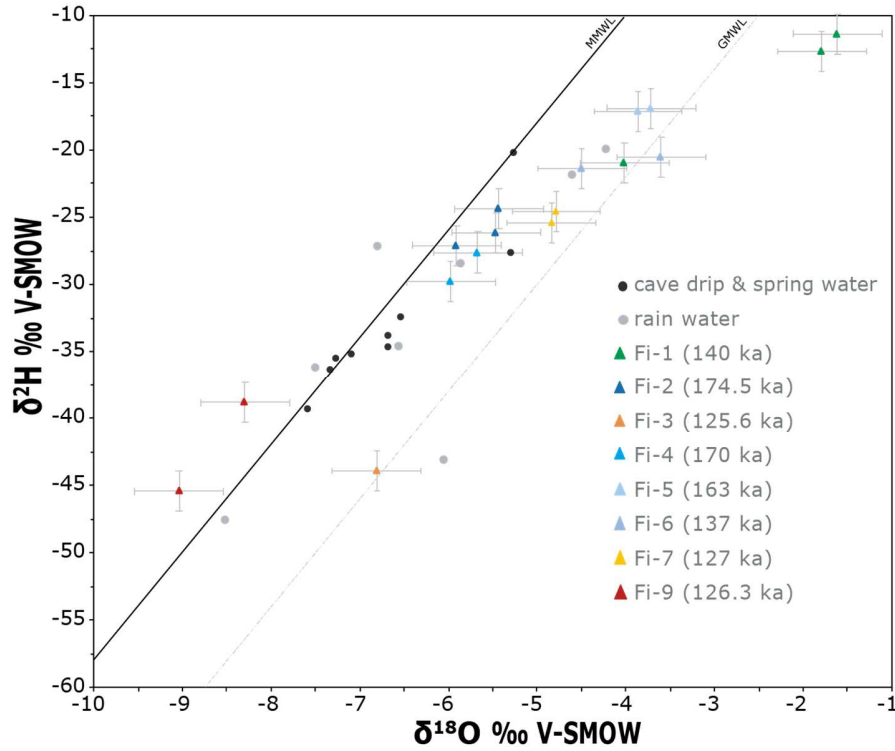
Figure 9. \delta^{18}\text{O} and \delta^2\text{H} values of 17 fluid inclusion samples from Pentadactylos stalagmite along with present-day dripwater and stream samples (this study) from the Kyrenia Range and rain water (IAEA/WMO, 2019) plotted on the MMWL (Gat et al., 2003) and GMWL (Rozanski et al., 1993).
