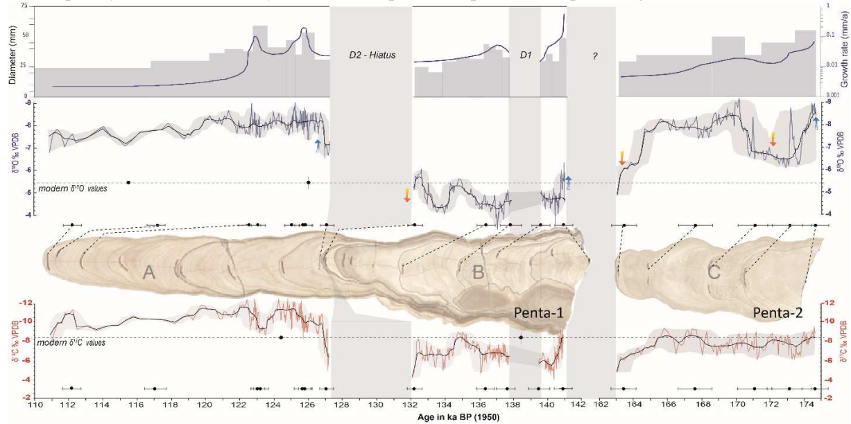
Figure 4. \delta^{18}\text{O} and \delta^{13}\text{C} profiles of micro-drilled samples along the growth axis of Pentadactylus Cave stalagmite (Cyprus) reported with their radiometric age. The original isotopic data are presented with their moving average (black line) to clearly show the general trend in isotopic variations from 163 to 174 ka (Penta-2) and from 112 to 141 ka (Penta-1). The period from 138 to 140 ka is not displayed as no isotopic measurements were made for this period. The isotopic changes are displayed relative to V-PDB (Vienna Pee Dee belemnite) together with growth rate (mm/a) and stalagmite diameter (mm). The modern \delta^{18}\text{O} and \delta^{13}\text{C} values represent calcite samples retrieved under active seepage water from the cave. Blue arrows show wet phases and yellow arrows refer to dry phases.
