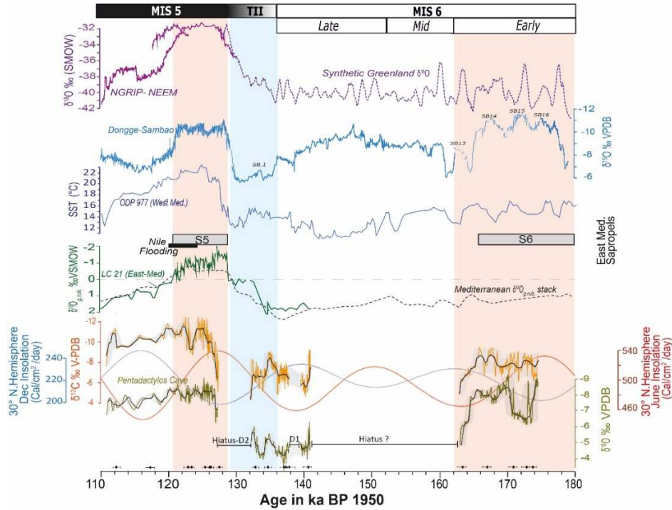
Figure 6. Marine and global records from 110 to 176 ka excluding the period from 142 to 162 ka (white column) and compared to the Pentadactylos \delta^{18}\text{O} profile (this study). Marine and global records comprise \delta^{18}\text{O} Greenland ice core (NGRIP, 2004 ; NEEM, 2013) with the synthetic \delta^{18}\text{O} record (Barker et al., 2010), Sambao-Dongge \delta^{18}\text{O} profile in central China (Wang et al., 2008, Cheng et al., 2016), SST ( ^{\circ}\text{C} ) in ODP 977 marine core (Martrat et al. 2004, 2014), \delta^{18}\text{O}_{\text{g.rub}} in LC21 marine core (Grant et al., 2012, 2016) and Mediterranean \delta^{18}\text{O}_{\text{g.rub}} stack (Wang et al., 2010), Sapropels S6 and S5 (Ziegler et al., 2010) and the July insolation at 30^{\circ}\text{N} (Berger and Loutre, 1991).
