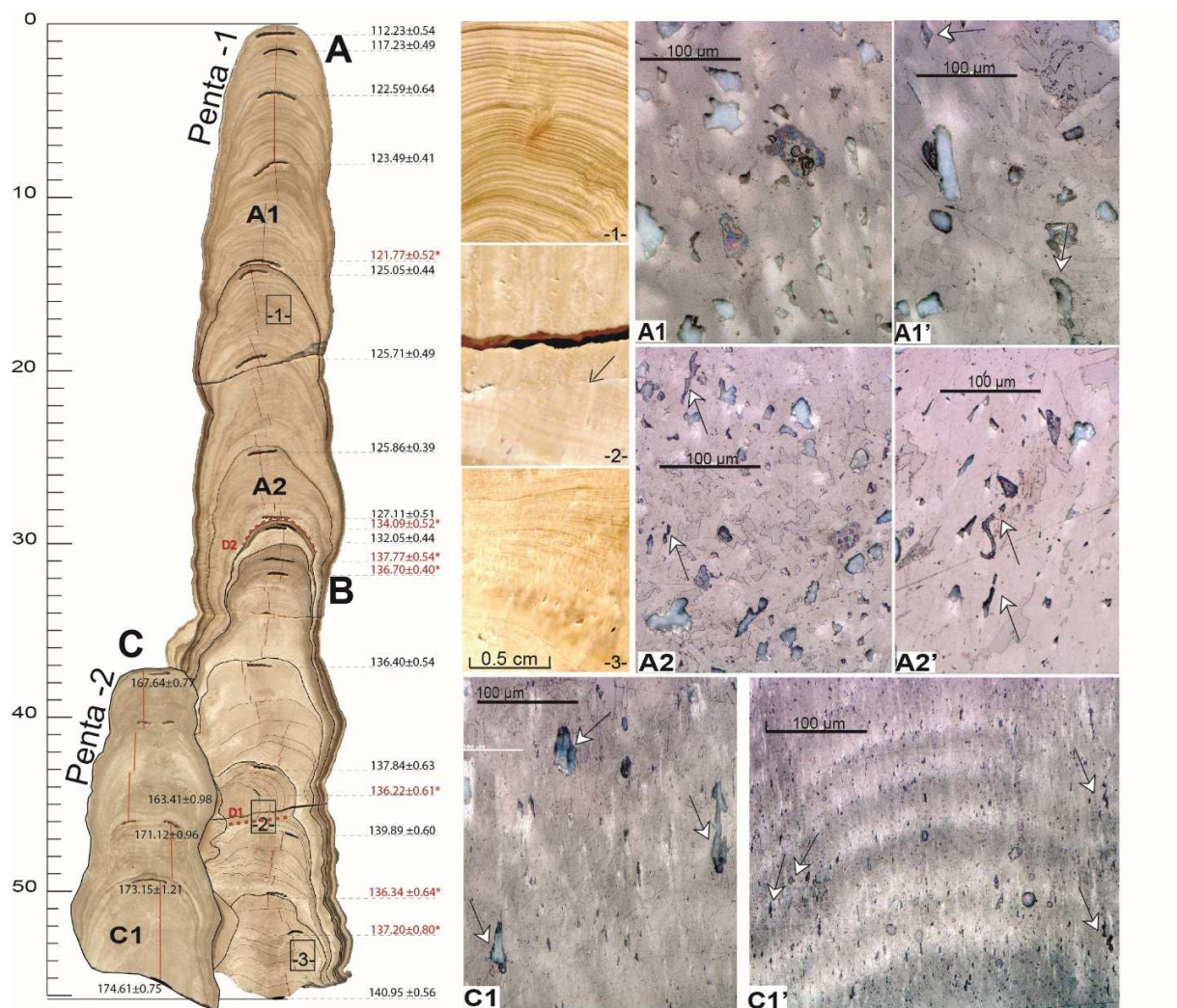
Figure 2. Petrographic sections of the speleothem Penta-1 and Penta-2 showing from left to right: an image scan of the speleothem, the stable isotopes sampling track (red line), the location of the U–Th datings, location of photos 1, 2 and 3 showing the structure of the calcite laminae at 15 cm (photo 1), 46 cm (photo 2) and 53 cm (photo 3) depths. Locations of A1, A2 and C1 microscope images along the speleothem growth axis, are thin section photos with an indication of the identified large fluid inclusions (arrows). Discontinuities D1 and D2 as well as ages considered outliers are marked in red.
