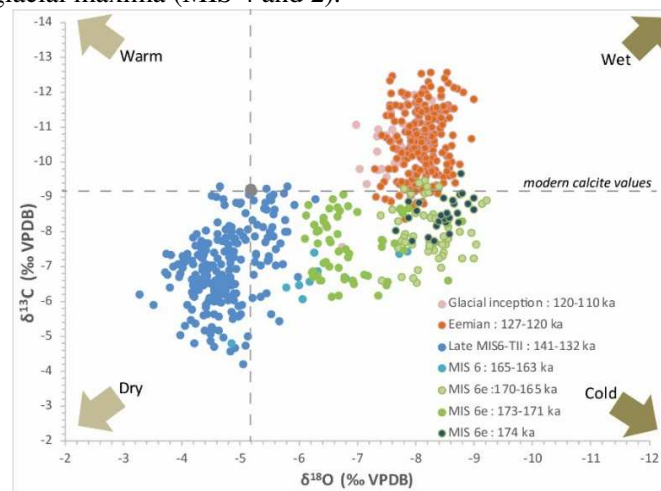
Figure 5. cross plot of the stable isotope values from Pentadactylos Cave covering the early-MIS 6, the late-MIS 6-TII, the MIS 5e (Eemian), the glacial Inception and modern (late-Holocene) periods. VPDB, Vienna Pee Dee belemnite.
