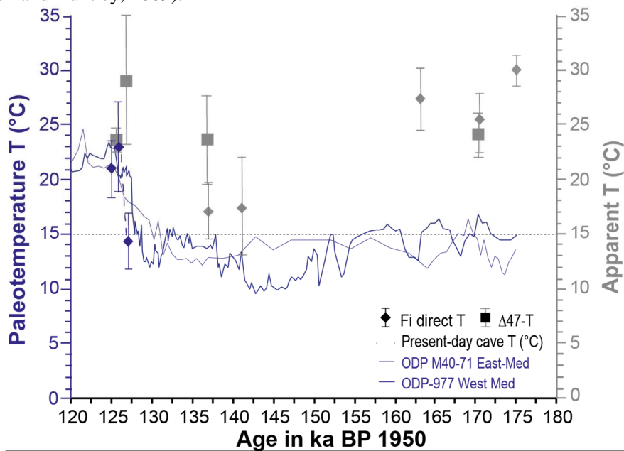
Figure 10. Paleotemperatures based on the fractionation ^{18}\alpha(\text{CaCO}_3\text{-H}_2\text{O}) from fluid inclusion values (in blue) before 130 ka with the apparent T from clumped isotopes analysis (grey squares) based on the \Delta_{47}\text{-}T calibration of Kluge et al. (2015). Temperatures are plotted against the present-day cave temperature and the SST (blue lines) from the nearby marine cores (M40-71 from Emeis et al., (2003) and ODP-977 from Martrat et al., (2014). Fluid inclusion T that are assumed to be influenced by evaporation are shown as small grey triangles.
