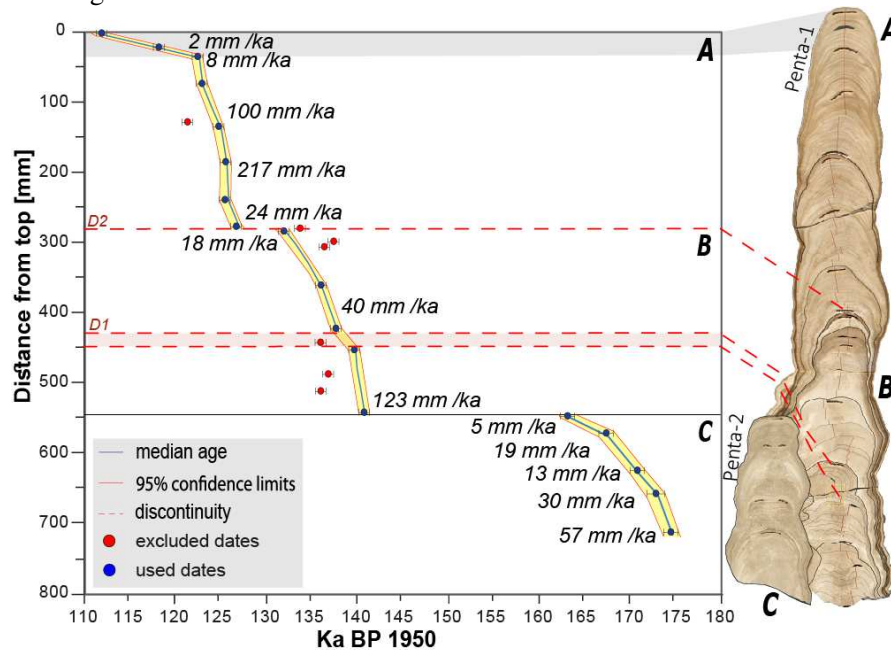
Figure 3. Age model of the Pentadactylos record. Growth rate of the stalagmite is given next to the age model using COPRA polynomial statistics model between two consecutive dates.
