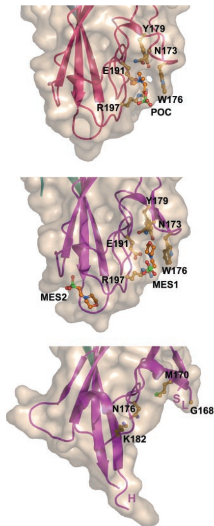
FIG. 4. Structural variation in the rim domain of leucotoxins and lipid binding capability. Ribbon and semi-transparent surface representation comparing the rim domains of HlgB ( top panel ), LukF-PV ( middle panel ), and LukS-PV ( bottom panel ). The phosphocholine headgroup of DiC_3PC (POC) and MES molecules as well as residues defining the corresponding binding sites in HlgB and LukF-PV, respectively, are shown and labeled. Carbon, nitrogen, oxygen, and phosphorus (or sulfur) atoms are orange, blue, red, and green, respectively. The binding of POC (MES) is mainly mediated by hydrophobic/van der Waals' contacts and involves a single polar interaction between the main chain nitrogen atom of residue Arg-197 and an oxygen atom of the phosphate (sulfonate) group.
