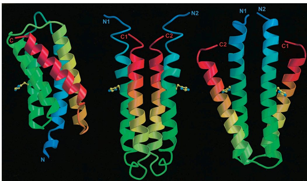
FIG. 8. Phosphoaccepting domains from CheA, EnvZ, and Spo0B. Left, S. typhimurium CheA-P1; Middle, E. coli EnvZ dimerization domain (PDB entry code 1JOY); Right, B. subtilis Spo0B dimerization domain (1IXM). The color of each polypeptide chain varies from dark blue (N termini) to red (C termini). The four-helix bundles of EnvZ and Spo0B result from dimerization. The N and C termini of these subunits are labeled. The structures are oriented such that one active site histidine residue (ball-and-stick) and the helix to which it belongs have similar positions and orientations. The figure was produced with BOBSCRIPT (59) and rendered in RASTER3D (60).
