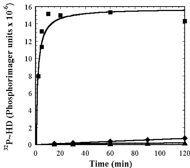
FIG. 6. Time course of CheA-P1 phosphorylation by ATP. A solution containing 100 \mu M of wild-type CheA-P1 (■) or the mutants K51A (◆) or E70A (▲) were incubated at 24 °C in the presence of 10 \mu M CheA catalytic domain and [ \gamma - ^{32} P]ATP. Aliquots were taken at the indicated times and analyzed as described under “Experimental Procedures.”
