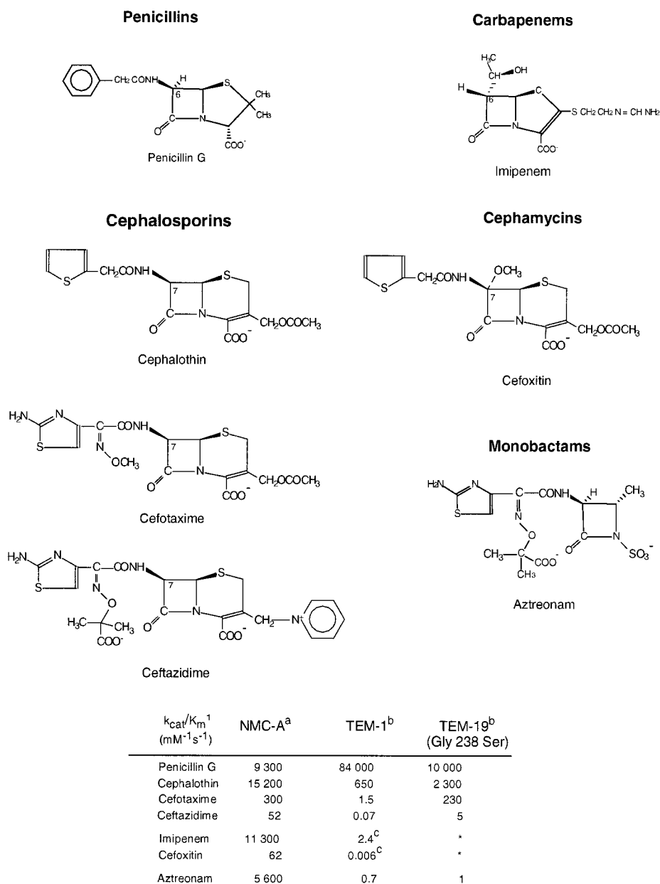
FIG. 1. Chemical structures of the five classes of \beta -lactam antibiotics. The letters a , b , and c indicate kinetic data from Refs. 16, 42, and 17, respectively. *, not measurable.
