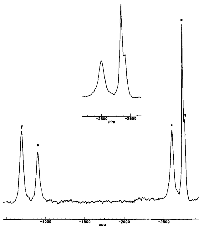
Figure 4. ^{59}\text{Co} NMR spectrum of the reaction mixture of 2a with \text{Me}_3\text{NO} : (●) 2a , (▼) \text{HFeCo}_3(\text{CO})_{10}(\text{NMe}_3)_2 , (*) [\text{FeCo}_3(\text{CO})_{12}]^- (–2597 ppm).
