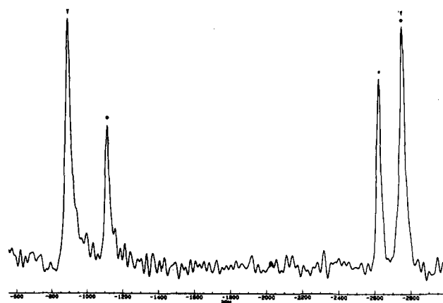
Figure 3. ^{59}\text{Co} NMR spectrum of the reaction mixture of 2b with \text{Me}_3\text{NO} : (●) 2b , (▼) \text{HRuCo}_3(\text{CO})_{10}(\text{NMe}_3)_2 , (*) [\text{RuCo}_3(\text{CO})_{12}]^- (–2617 ppm).
