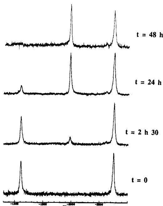
Figure 2. ^{59}\text{Co} NMR monitoring of the reaction of 2b with \text{SET}_2 in \text{CDCl}_3 showing the formation of 6b : reaction time t = 0 , pure 2b ; t = 48 h, pure 6b .
