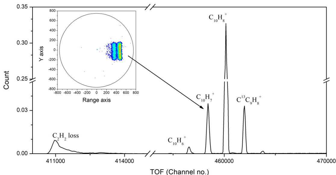
Fig. 2. ToF spectrum of az recorded at 235nm and 9 \times 10^9 W/cm 2 . Inset figure corresponds to the distribution of H loss channel on ion PSD. It separates low and high energy H loss peaks along the horizontal coordinate with a typical resolution of 7eV over 3keV.
