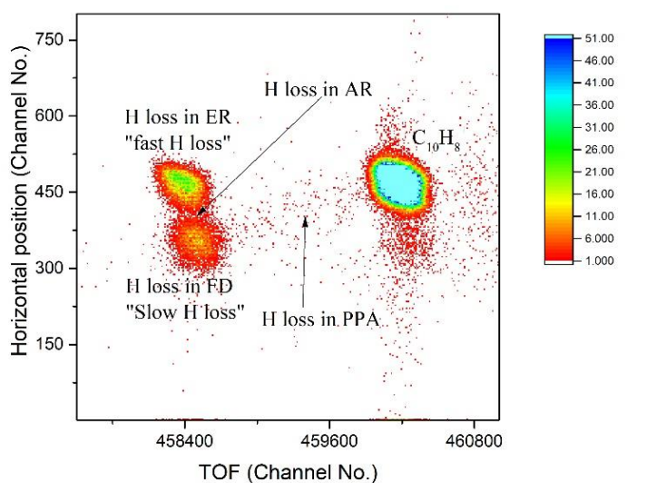
Fig. 3. 2D diagram for ToF vs horizontal position (horizontal position linearly scale to the kinetic energy of the ion) of parent and H loss fragment ion measured at 235nm and 9 \times 10^9 W/cm 2 . Various features in the 2D diagram are marked according to their corresponding decay location.
