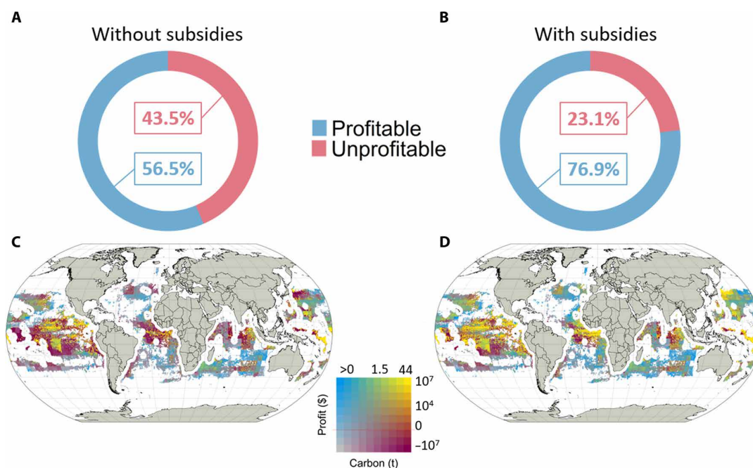
Fig. 3. Impact of government subsidies on blue carbon extraction in the high seas. Percentage of blue carbon extracted in profitable areas and unprofitable areas without subsidies (A) and with subsidies (B). Spatial variability of carbon extraction and economic viability without subsidies (C) and with subsidies (D).
