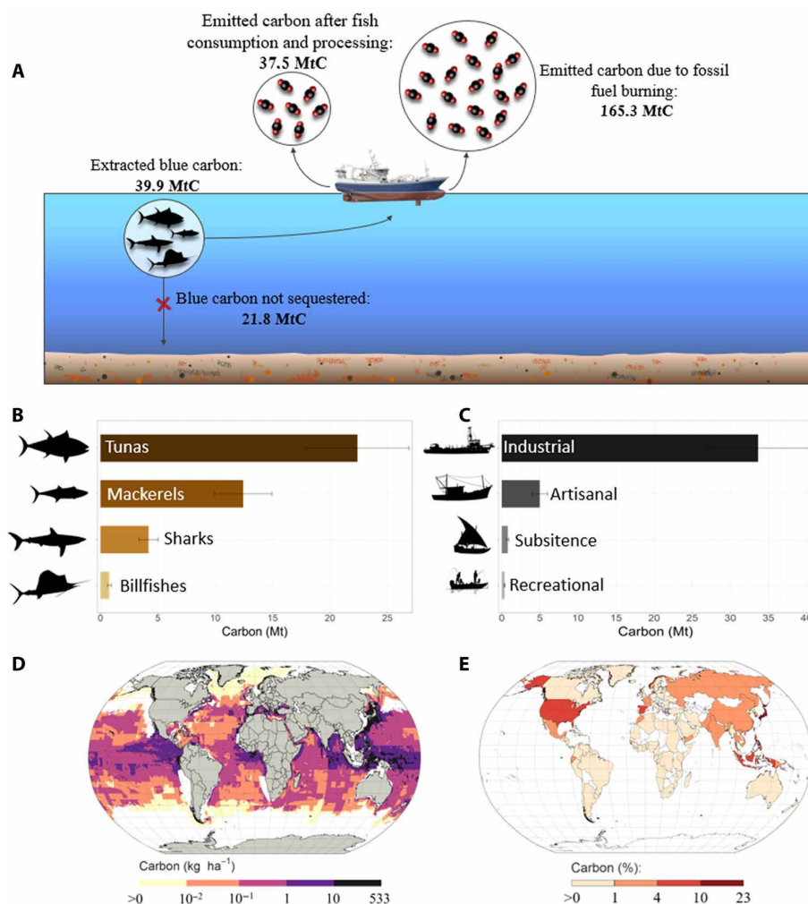
Fig. 1. Total blue carbon extraction of large fish since 1950. Fate of blue carbon and associated emissions ( A ). Blue carbon extracted by taxon ( B ) and by fishing sector ( C ). Error bars represent the lower and upper bounds of carbon content in fish bodies (10 and 15%, respectively). Spatial distribution of the blue carbon extracted since 1950 by fisheries ( D ). Percentage of countries' contribution to blue carbon extraction since 1950 ( E ). Countries in white have no reported catches.
