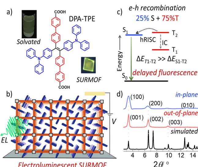
Figure 1. a) Chemical structure of DPA-TPE linker and its turn-on emissive feature in SURMOF state; b) electroluminescence (EL) in the DPA-TPE based SURMOF, enforced by coordination and periodic stacking; c) energy diagram of the singlet (S) and triplet (T) states of DPA-TPE in SURMOF, demonstrating "hot exciton" reverse intersystem crossing (hRISC) process; d) simulated and experimental out- and in-plane x-ray diffraction patterns of Zn-DPA-TPE (1).
