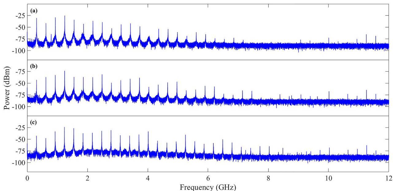
FIG. 5. (a)–(c) The respective FFT spectra corresponding to the intensity traces shown in Fig. 4.
