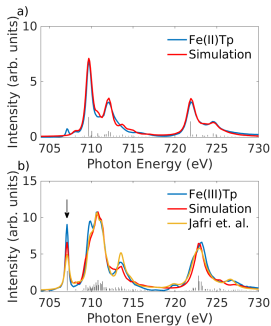
Figure 5: L 2,3 -edge XAS spectra (thick solid blue lines) of K 2 [Fe II (Tp)(CN) 3 ] (a) and Li[Fe III (Tp)(CN) 3 ] (b) measured at 200 K, with charge transfer multiplet simulations (red and orange solid lines). The red lines represent the result of multiplet simulation fits to XAS spectra and the vertical sticks represent the individual transition intensities. The orange line in (b) represents the results of simulations published by Jafri et. al. in Ref 22. The black arrow at the low energy side of the L 3 edge is characteristic of low spin 3d 5 .
