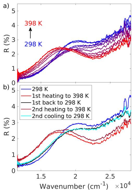
Figure 2: Solid-state UV-vis reflectance spectra of Fe 42 , (a) measured as a function of temperature and (b) reversibility in the shifting of bands on repeated heating and cooling cycles.
