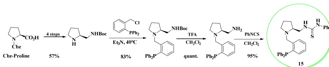
Scheme 9: Synthesis of thiourea-phosphine 15 from Cbz-proline.
