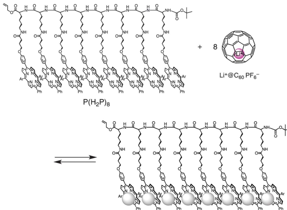
Figure 4. Supramolecular formation of peptide porphyrin oligomers with Li^+@C_{60} . Ar = 3,5-di- tert -butylphenyl.
