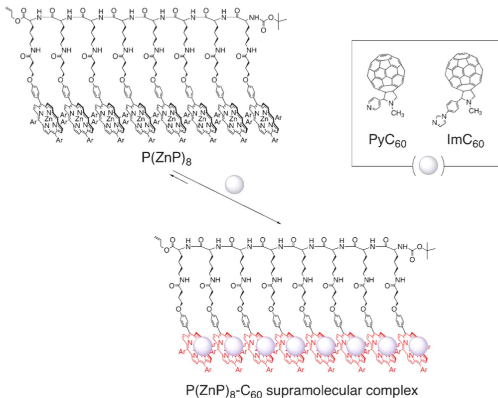
Figure 2. Illustration of a supramolecular complex composed of the porphyrin–peptide octamer P(\text{ZnP})_8 and \text{PyC}_{60} or \text{ImC}_{60} . Ar = 3,5-(t-Bu) _2\text{C}_6\text{H}_3 .
