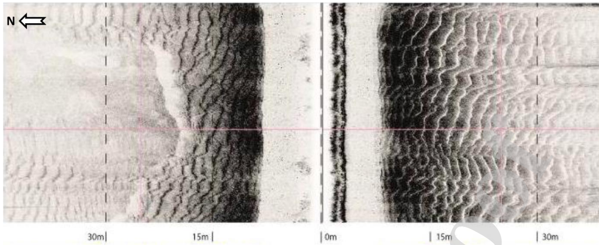
Figure 5. Side-scan sonar images of flood-dominant bedforms in the main Maroni channel (see 2 in Fig. 3; with kind permission from the Bureau de Recherches Géologiques et Minières, 2019).
