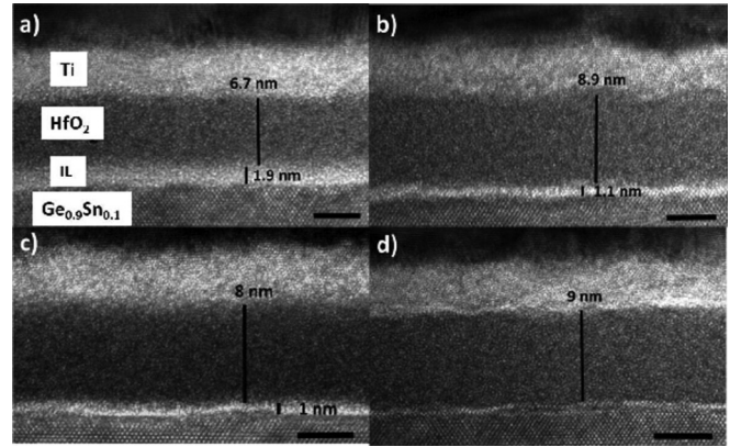
FIG. 1. Cross-sectional HR-TEM images of (a) S1, 1 nm- \text{GeSnO}_x /1 nm- \text{Al}_2\text{O}_3 /7 nm-HfO 2 , (b) S2, 1 nm- \text{Al}_2\text{O}_3 /9 nm-HfO 2 , (c) S3, 1 nm- \text{GeSnO}_x /8 nm-HfO 2 , and (d) S4, 9 nm-HfO 2 gate stacks. The scale bars are 5 nm for all images.
