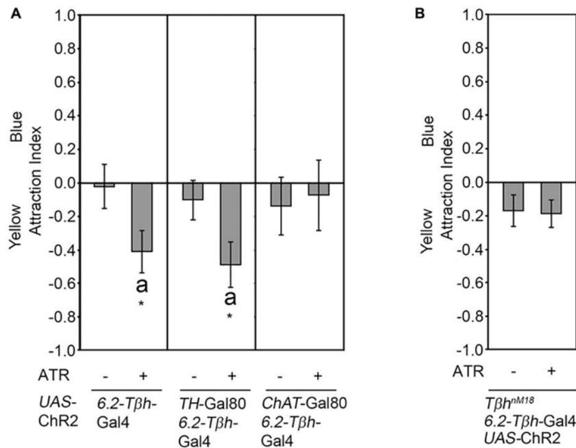
FIGURE 2 | Octopamine release causes aversion. (A) Neuronal activation under the control of the 6.2-Tβh-Gal4 driver elicits site aversion (AIs of the control and experimental group: 0.02 \pm 0.14 and -0.41 \pm 0.13 , respectively; n = 22, 19 ). Removal of the activation of dopaminergic neurons by combining the 6.2-Tβh-Gal4 driver with the TH-Gal80 driver does not influence aversion (AIs for the control and experimental group: 0.1 \pm 0.12 and -0.49 \pm 0.14 , respectively; n = 14, 14 ). Removing ChAT positive neurons by using the ChAT-Gal80 in combination with the 6.2-Tβh-Gal4 driver resulted in loss of aversion (AIs of control and experimental group: -0.14 \pm 0.17 and -0.08 \pm 0.21 respectively; n = 13, 11 ). (B) Activation of the UAS-ChR2 transgene under the control of 6.2-Tβh-Gal4 in Tβh M18 mutants eliminates aversion (AIs of the control and experimental group: -0.17 \pm 0.1 and -0.19 \pm 0.08 , respectively; n = 20, 19 ). For activation, the flicker frequency of 2 s at 40 Hz, 16 s at 8 Hz and 2 s at 0 Hz was used. Errors are SEM. Differences from random choice were determined using the one-sample sign test and are indicated by the letter “a”. Student’s T -test was used to determine differences between two groups. * P < 0.05 . For data, see Supplementary Table S2 .
