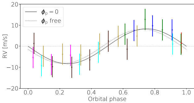
Figure 4. Activity-subtracted RV time-series (dots) folded to P_{\text{orb}} using T_0 as reference time. The subtracted activity RV signal is estimated assuming \phi_p = 0 and S = 0 \text{ m s}^{-1} . Data points of same colour belong to the same orbital phase. We plot in solid and dotted black lines, the planet RV signatures obtained assuming \phi_p = 0 and optimizing \phi_p in the MCMC process, respectively.
