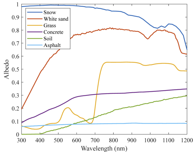
Fig. 3. Spectral albedo of the six materials considered.
