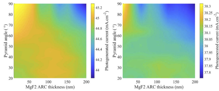
Fig. 13. Simulated photogenerated currents in the bifacial tandem (left is structure (d) and right structure (b)) module as a function of back glass texture pyramid base angle and ARC thickness. The device is illuminated by direct AM1.5 g spectrum at the front and diffuse light coming from sand (left) and grass (right) albedo.
