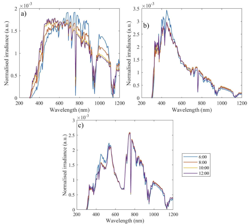
Fig. 14. Denver averaged irradiation spectra computed over a year, grouped by hour of the day. Direct normal irradiance (A), diffuse irradiance on a tilted surface (B) and diffuse irradiance reflected by grass albedo (C) are modelled. Spectra are all normalized to a broadband power of 1 \text{ W}\cdot\text{m}^{-2} in order to compare their shapes.
