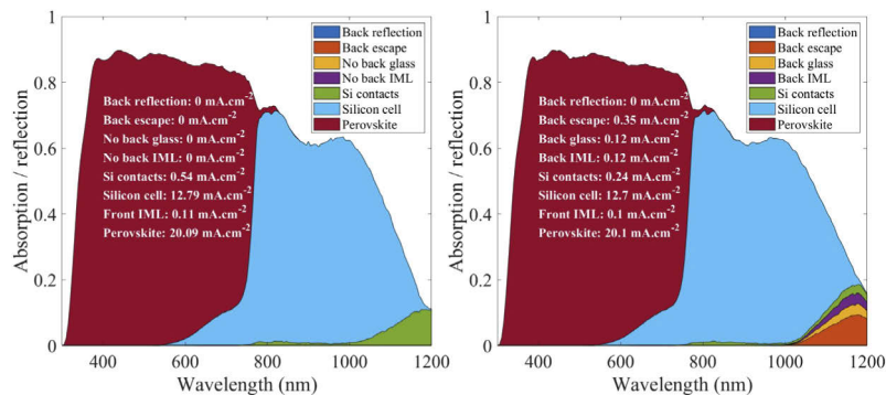
Fig. 12. Absorption simulated in modules. Currents are also shown in order to help analyzing losses at the back of the silicon cell for the monofacial (left) and bifacial module (right). In this case incoming light only comes from the front.
