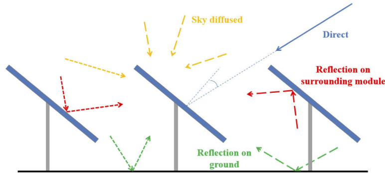
Fig. 2. Decomposition of the irradiance perceived at the front and back sides of a photovoltaic module in a field configuration.
