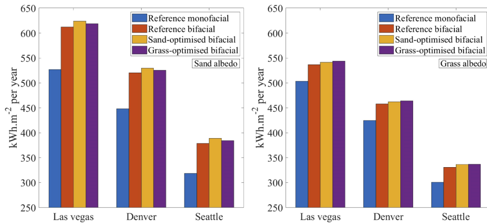
Fig. 10. Energy production estimation in realistic conditions at three locations for sand (left) and grass (right) albedo. Reference modules are presented in Fig. 1, enhanced bifacial devices are presented in Fig. 6(b) and (d).
