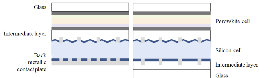
Fig. 1. Monofacial (left) and simple bifacial (right) module structure. For the bifacial module the back silicon contact grid is modified, IML and a glass layer are added.
