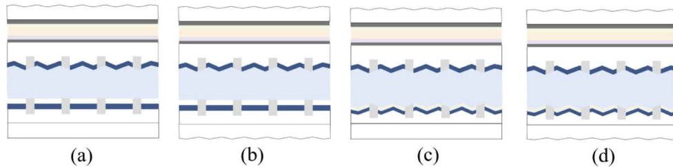
Fig. 6. Structure of the modeled bifacial modules. Modules with either: no silicon and glass back-side texture (a), only glass back texture (b) or silicon back texture (c), or both glass and silicon back-side textures (d) are investigated.
