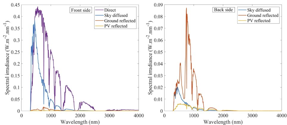
Fig. 8. Spectral irradiance perceived at the front side (left) and back side (right) of a photovoltaic module. Spectra are averaged over a year. Location is Denver and a grass albedo is considered. PV reflected is the component that is reflected on the facing module (see Fig. 2).
