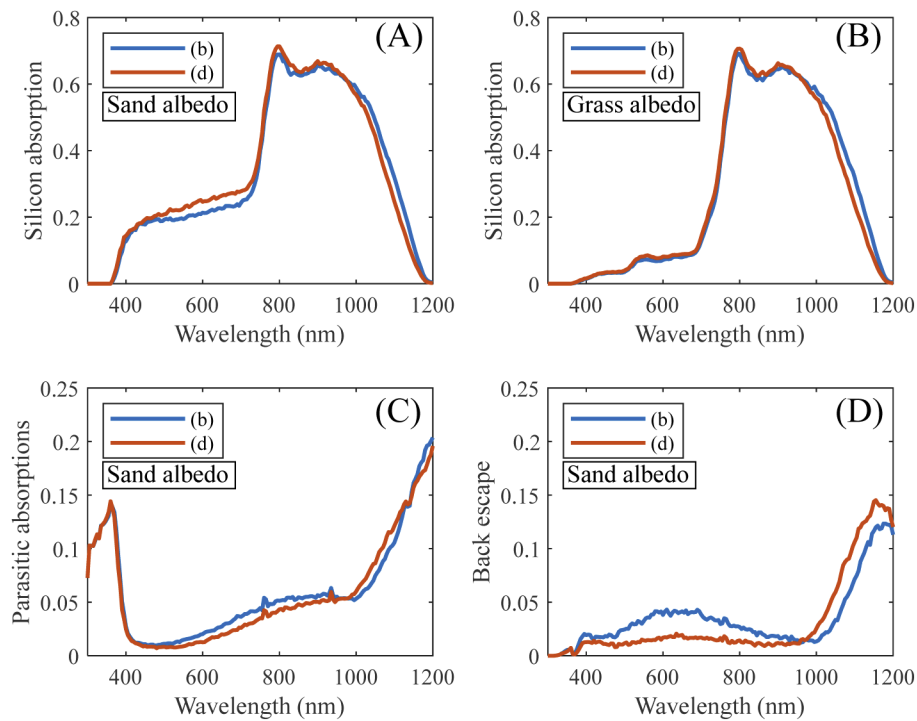
Fig. 7. Silicon absorption in bifacial devices: (A) and (B). Parasitic absorptions in back silicon dielectrics, IML and glass: (C), and escaping light through the back of the devices: (D). Direct AM1.5 g spectrum at the front and diffuse light coming from sand albedo: (A), (C) and (D), or grass albedo: (B). Devices have only a glass texture (b) or both glass and silicon textures (d).
