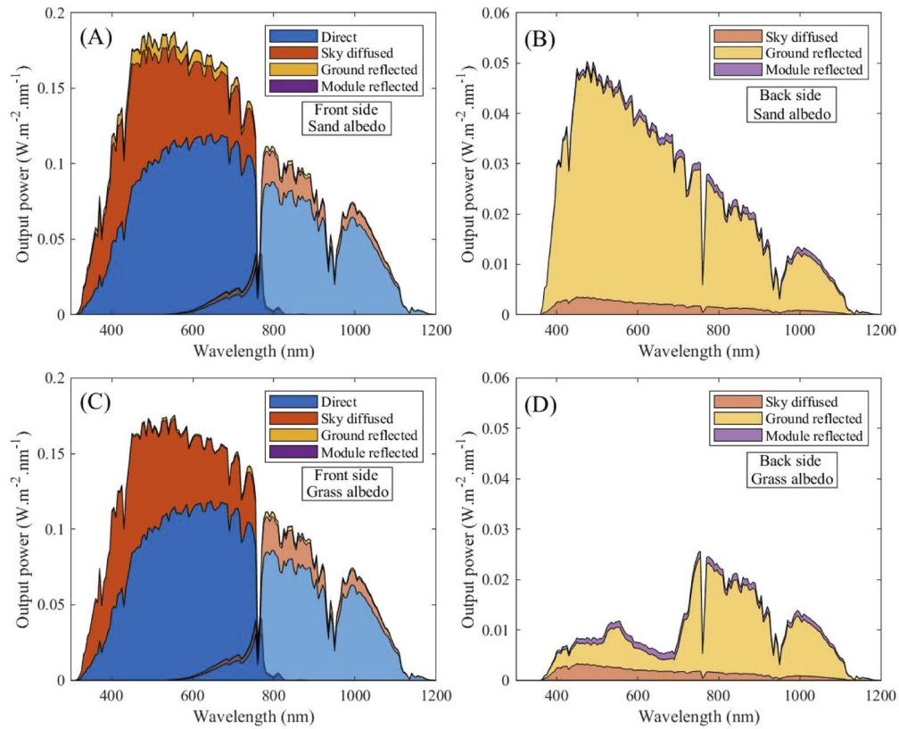
Fig. 9. Spectral output power of the perovskite cell (dark colors) and the silicon cell (light colors). The considered module is optimized for strong albedo conditions (d) in Fig. 6). Average irradiance spectra from Denver with a sand albedo (a) and b) or a grass albedo (c) and d) are considered. a) and c) show the front side, b) and d) the back side.
