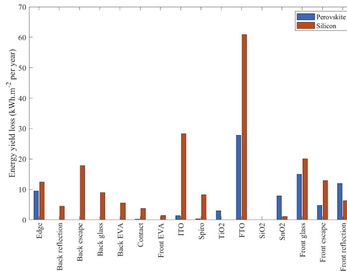
Fig. 11. Energy yield reduction through optical losses in both sub-cells. Realistic conditions in Denver with a sand albedo are used. Perovskite and Silicon refers to losses occurring respectively above or below perovskite bandgap.
