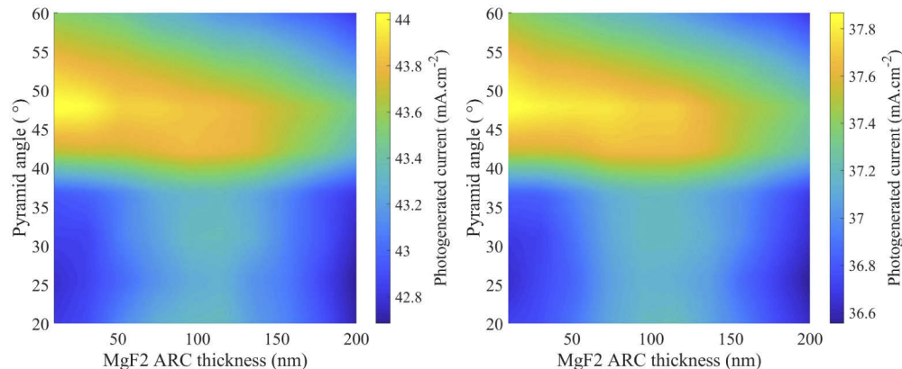
Fig. 5. Photogenerated current in the bifacial tandem module as a function of front glass texture pyramid base angle and ARC thickness. The module is illuminated by direct AM1.5 g spectrum at the front and diffuse light coming from sand (left) and grass (right) albedo.
