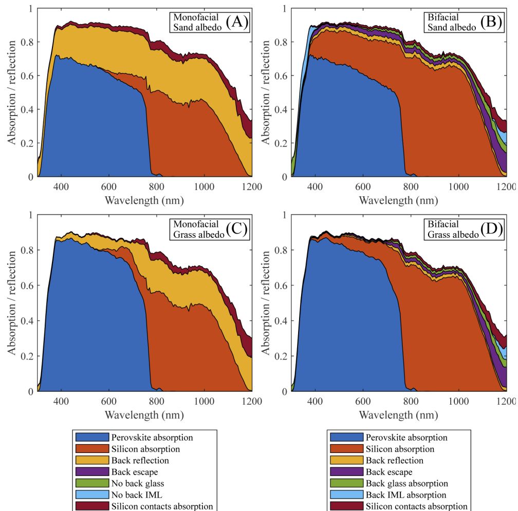
Fig. 4. Absorption, reflection and loss analysis. Monofacial module with sand (A) and grass (C) surrounding albedo, bifacial module with sand (B) and grass (D) surrounding albedo. Front irradiation is direct AM1.5 g spectrum in all cases. Back irradiation with diffuse light, is considered in both cases for the sake of comparison explaining the “Back reflection” area in the monofacial case.
