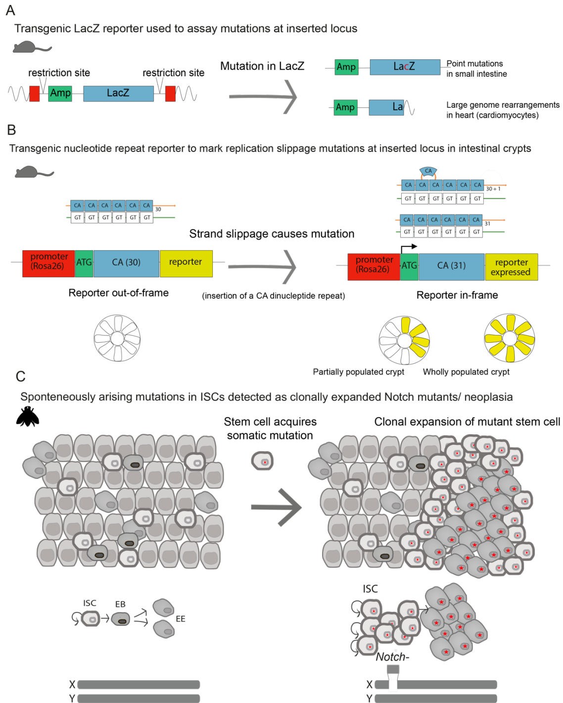
Figure 4. The use of model systems to assay spontaneous mutations in adult tissues. (A) A LacZ reporter to assay spontaneous mutations (Dolle et al. 2000). In this assay, genomic DNA extracted from young/old hearts and small intestines of transgenic mice containing the LacZ reporter is assessed for spontaneous mutation. LacZ encoding plasmids are recovered in bacteria tested for intact LacZ activity. A significant age related increase in point mutations was detected in small intestines whereas a significant age related increase in genomic rearrangements was detected in hearts. (B) A transgenic nucleotide repeat reporter assay to mark spontaneous mutations in mouse
