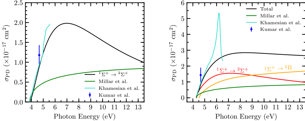
Figure 1: Photodetachment cross sections of \text{CN}^- (left panel) and \text{C}_3\text{N}^- (right panel).
