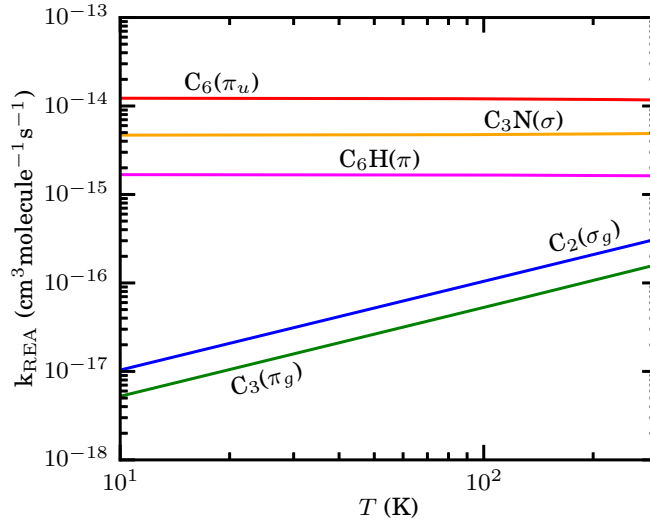
Figure 2: DREA rate coefficients for selected molecules. The symmetry of the Dyson orbital is indicated for each molecule.
