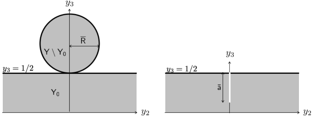
Fig. 8 Section Y of the defect in the two examples. Left: case of a stiffening by a circular cylinder; Right : case of a weakening by a transverse crack. By symmetry, there exists the same cylinder or the same crack in the opposite side y_3 < 0 .
