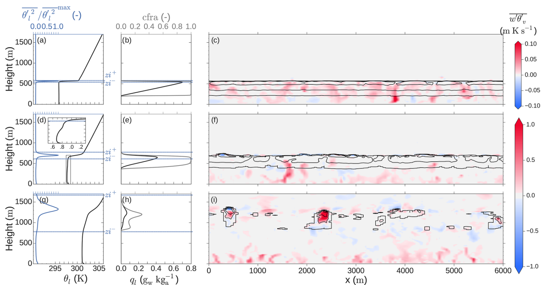
Figure 3. On the left (a, d, g), slab-averaged vertical profile of liquid potential temperature \theta_l (black) and \theta_l^2 normalized over its maximum value (blue). The inversion layer upper z_i^+ and lower z_i^- limits are indicated by dashed blue horizontal lines. In the center (b, e, h) slab-averaged vertical profiles of liquid water mixing ratio q_l (black) and horizontal cloud fraction cfra (grey). On the right (c, f, i), horizontal cross section of buoyancy flux \overline{w'\theta'_v} (red/blue) indicating upwards (downwards) movement of buoyantly positive (negative) air and cloud liquid water (in black contour lines every 0.3 \text{ g}_w \text{ kg}_a^{-1} ). Panels (a), (b) and (c) correspond to 05:00 UTC, (d), (e) and (f) to 11:00 UTC, and (g), (h) and (i) to 14:30 UTC. The inset in (d) is an expanded version of the rectangle in the same panel.
