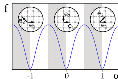
FIG. 1. Schematic representation of a lattice-invariant shear and the associated energy barriers along the simple shear loading path \boldsymbol{\gamma} = \mathbb{1} + \alpha \mathbf{e}_1 \otimes \mathbf{e}_1^T . Alternating minimal-periodicity domains are marked in gray and white.
