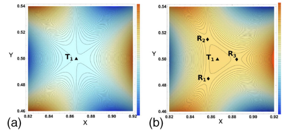
FIG. 6. Level sets of the energy density on the surface \det C = 1 around the point T_1 . We use the parametrization C_{11} = 1/y , C_{22} = (x^2 + y^2)/y , C_{12} = x/y . (a) Klein-invariant-based potential. (b) Polynomial potential (1) with \beta = -1/4 .
