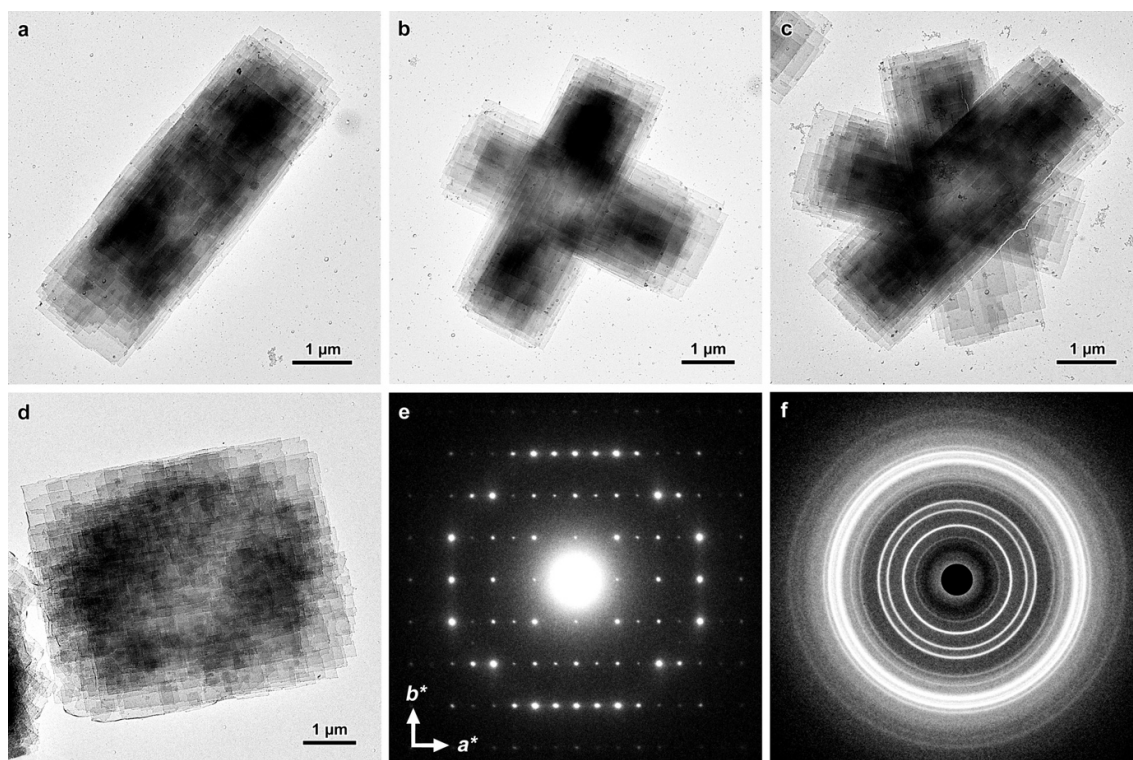
Fig. 2. The V_{6II} allomorph: a-d) TEM images of V-amylose crystallized with BBIOL (a-c) and HDIOL (d); e) base-plane ED pattern recorded at low temperature from a frozen-hydrated V_{BBIOL} crystal; f) XRD powder diagram recorded from V_{BBIOL} crystals equilibrated at 95% RH.
