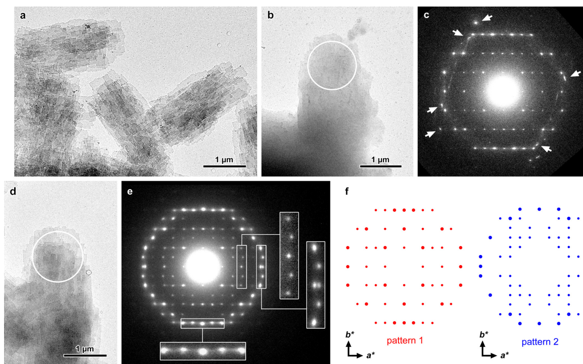
Fig. 9. a,b,d) TEM images of partially dried V_{\text{HDIOL}} crystals (a). In image b, a thin layer of mother liquor was frozen with the crystal, yielding extra spots (arrows) in the corresponding V_{6\text{II}} ED pattern (c). The lamellae are more clearly visible in the crystal in image d. In the corresponding ED pattern (e), some reflections are not in perfect alignment and others appear to be split (enlarged insets). The diagram is the superimposition of two patterns: pattern 1 (in red) is that of V_{6\text{II}} while pattern 2 (in blue) is similar to that of V_{7\text{II}} (f). However, the cell parameters calculated for pattern 2 are significantly smaller than those of V_{7\text{II}} . ED patterns c and e have been recorded from the selected areas indicated by white circles in images b and d.
