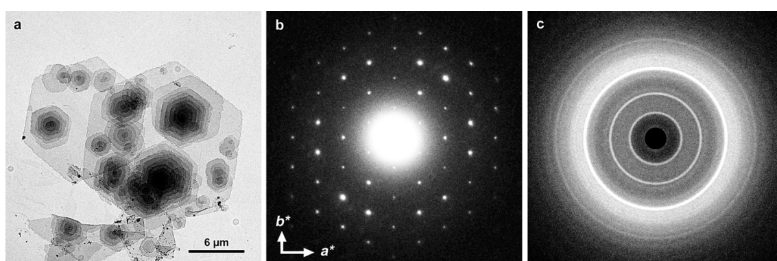
Fig. 3. The V_{7I} allomorph: a) TEM image of V-amylose crystallized with BBIOL; b) base-plane pseudo-hexagonal ED pattern recorded at low temperature from a frozen-hydrated crystal; c) XRD powder diagram recorded from crystals equilibrated at 95% RH.
