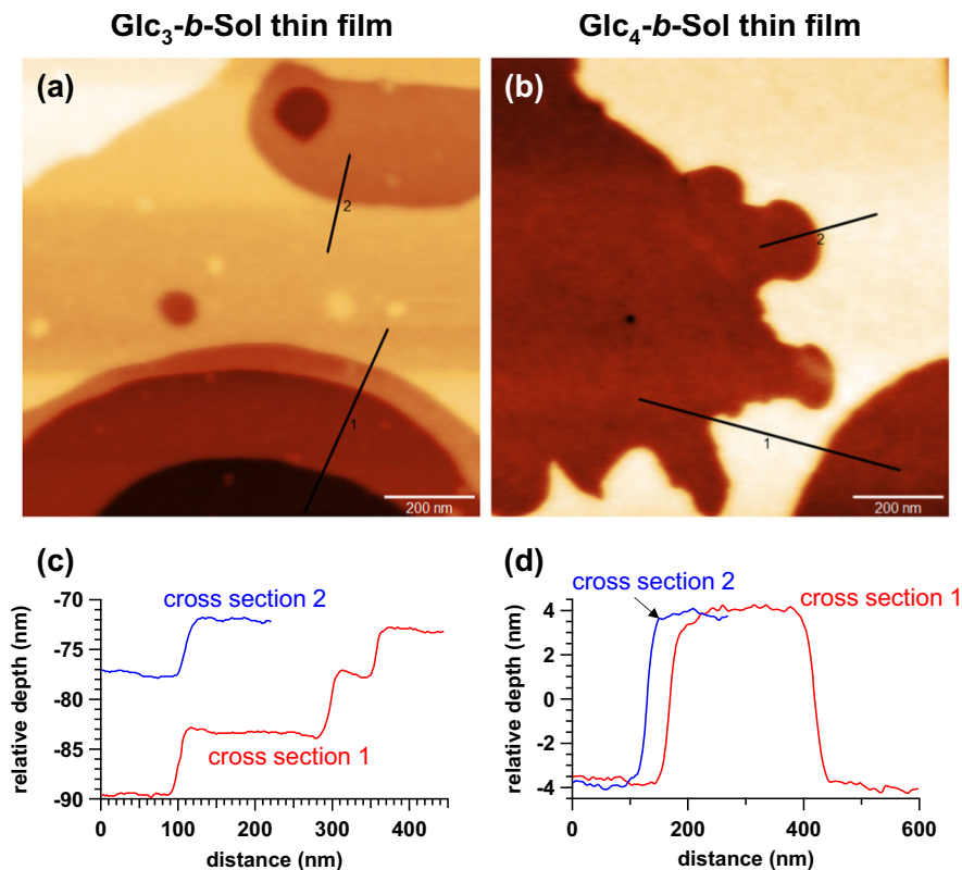
Fig. 4 Thin-film morphologies of \text{Glc}_3 - b -Sol and \text{Glc}_4 - b -Sol. AFM height images (a, b) and corresponding cross-sectional profiles (c, d) indicating the formation of 6–8-nm-thick horizontal lamellae in \text{Glc}_3 - b -Sol (a, c) and \text{Glc}_4 - b -Sol thin films (b, d). Thin-film samples were prepared by spin-coating the BCO solution onto the hydrophilic surface of a silicon substrate followed by thermal annealing at 85 °C for 1 h.
