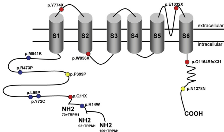
Figure 5. Localization of TRPM1 Mutations with Respect to Predicted Channel Domains The specific domains for the TRPM1 channel were estimated by the use of different publications and prediction programs 14,32 (UniProtKB-Swiss-Prot).
