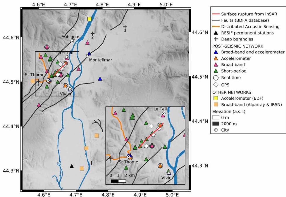
Figure 4. Location of seismicological and geodetic stations and Distributed Acoustic Sensing (DAS) measurement deployed in the field. Three deep boreholes are also indicated: Valvignières borehole (#1), Savasse borehole (#2) and Marsanne borehole (#3).
