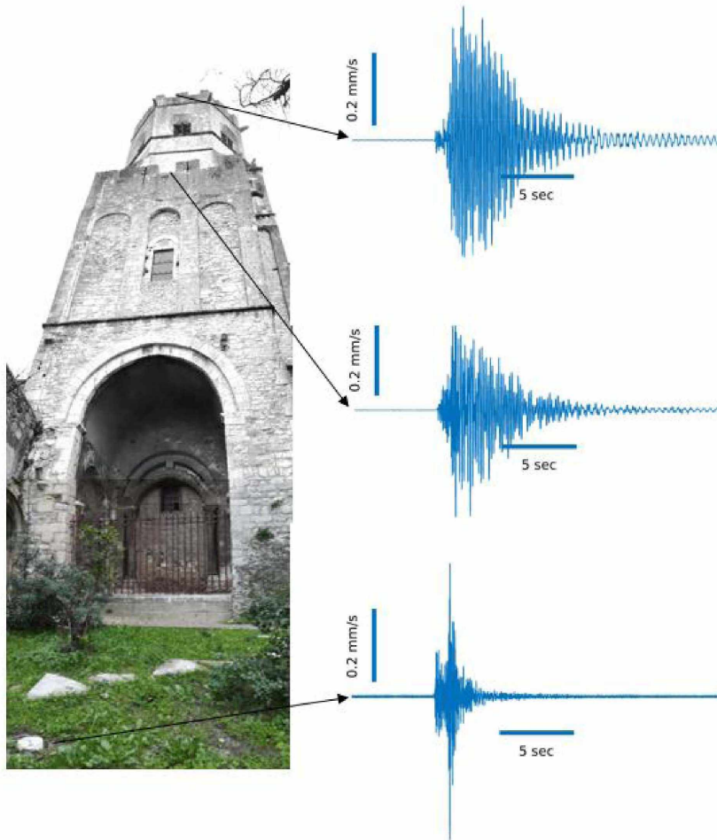
Figure 11. Velocities (NS component) recorded at different levels of the Saint Michel historical tower during the Ml 2 aftershock that occurred November 23, 2019.
