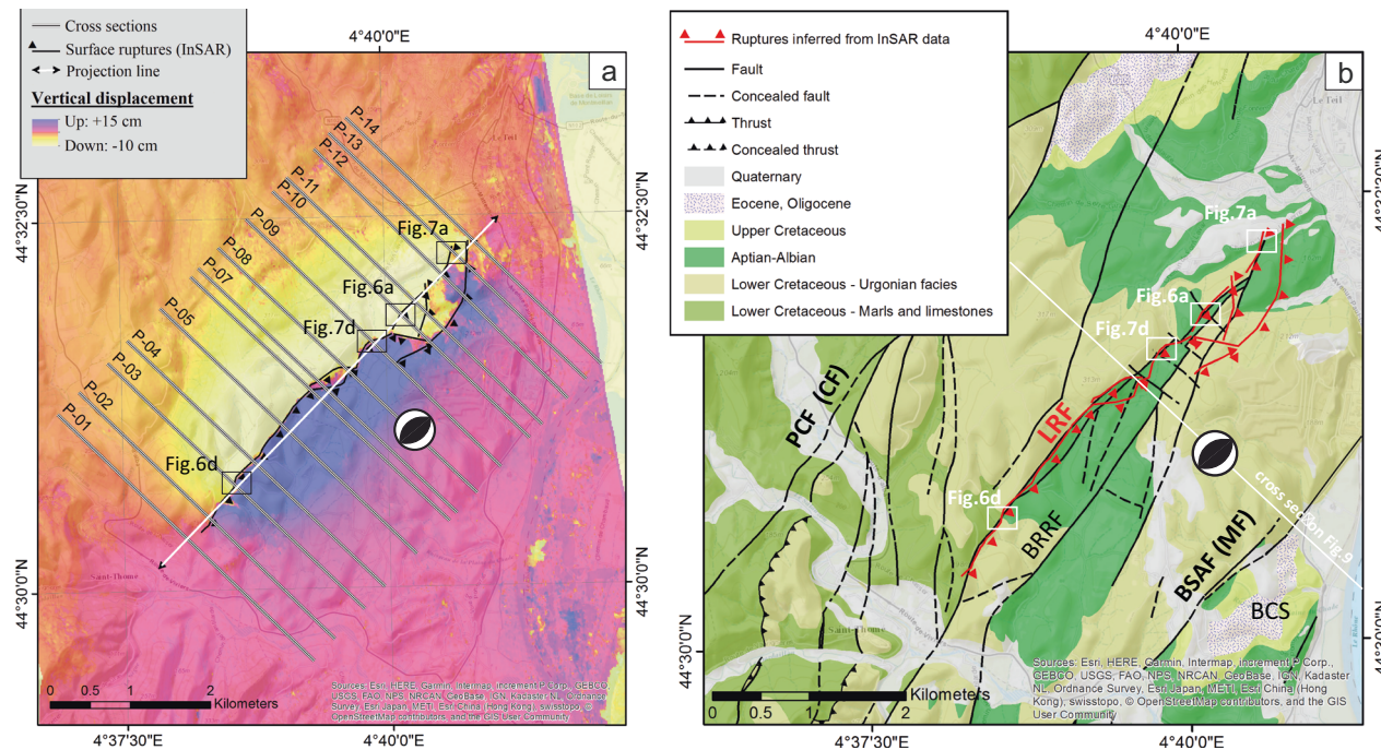
Fig. 4 Map of vertical displacements from InSAR data and map of the main geological formations in the region affected by the Teuil earthquake. a Vertical displacement associated to the 11 November 2019, M_w 4.9 Le Teuil earthquake inferred from the unwrapped InSAR interferogram (ascending track) draped over a satellite image of the area; maximum gradient on this map allows tracing the surface rupture; the epicenter of the event is represented by its focal mechanism; thin black lines correspond to extracted profiles across the rupture to determine the vertical displacement and the width of the deformation zone. b Simplified geological map (modified from BRGM) of the Le Teuil region highlighting the sharp correspondence between the co-seismic rupture trace inferred from InSAR (in red) and the La Rouvière Fault in black. PCF (CF) Pontet-de-Couloubre Fault (Cevennes Fault), LRF La Rouvière Fault, BRRF Bayne-Roche-Renard Fault, BSAF (MF) Bayne-Saint-Alban Fault (Marsanne Fault), BCS Bayne-Couij Janet Syncline.
