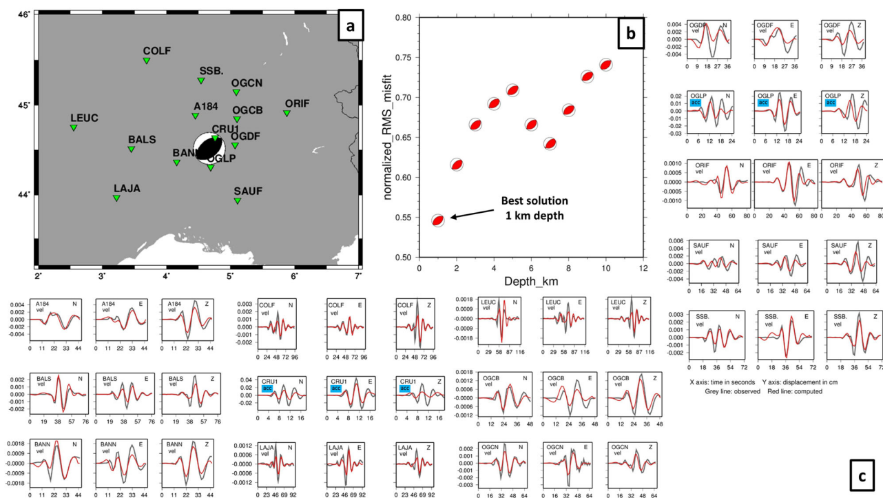
Fig. 2 Result of the waveform inversion. a Map with stations used (green triangles) and the focal mechanism corresponding to the best solution found. b Plot of focal mechanism solutions in an RMS versus depth graph. c Waveform fit, in displacement (cm) bandpass filtered between 0.03 and 0.08 Hz. Observed records are in gray and computed in red. For each station the three components are displayed (N, E, Z), and “vel” or “acc” (blue labels) means that the original record was in velocity (broadband) or acceleration (strong motion), respectively.
