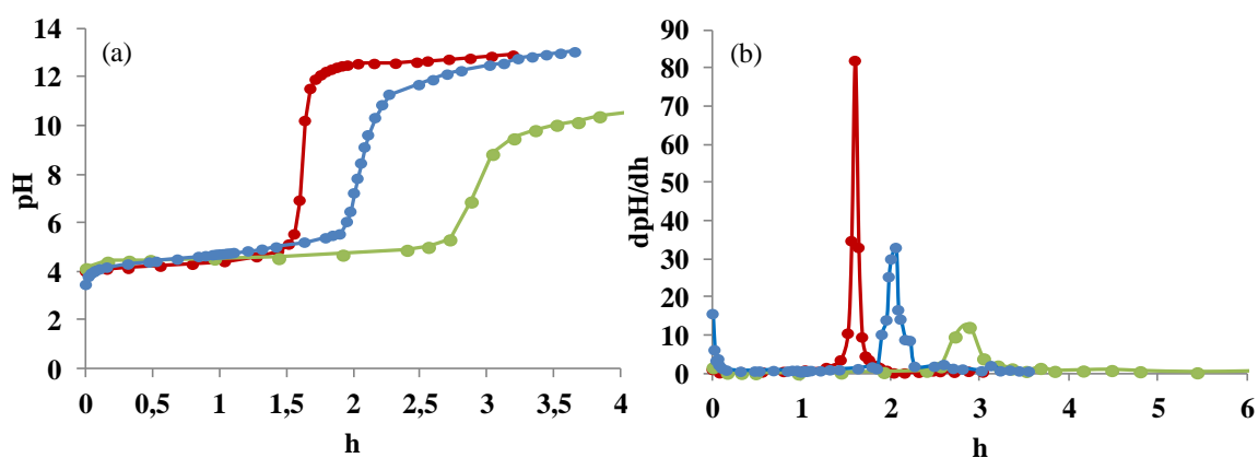
Figure S1: Evolution of the pH (a) and of dpH/dh (b) in function of h at R = 0 (without DHBC) during titration of Cu^{2+} ( 0.10 \text{ mol.l}^{-1} ) (●), Al^{3+} ( 0.05 \text{ mol.l}^{-1} ) (●) and (Cu^{2+} + Al^{3+}) ( 0.15 \text{ mol.l}^{-1} ) (●) by NaOH ( 0.2 \text{ mol.l}^{-1} ).
