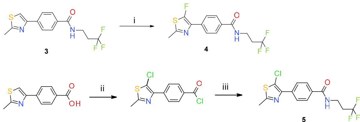
Figure 3. Synthesis of halogenated compounds 4 and 5. Reagents and reaction conditions: (i) Selectfluor (2.5eq.), anhydrous DMF, 0°C to RT, 55 h; (ii) SOCl 2 , 50°C, 6 h; (iii) 3,3,3-trifluoropropylamine hydrochloride (1.1eq.), DIEA (4eq.), DCM, RT, overnight.
