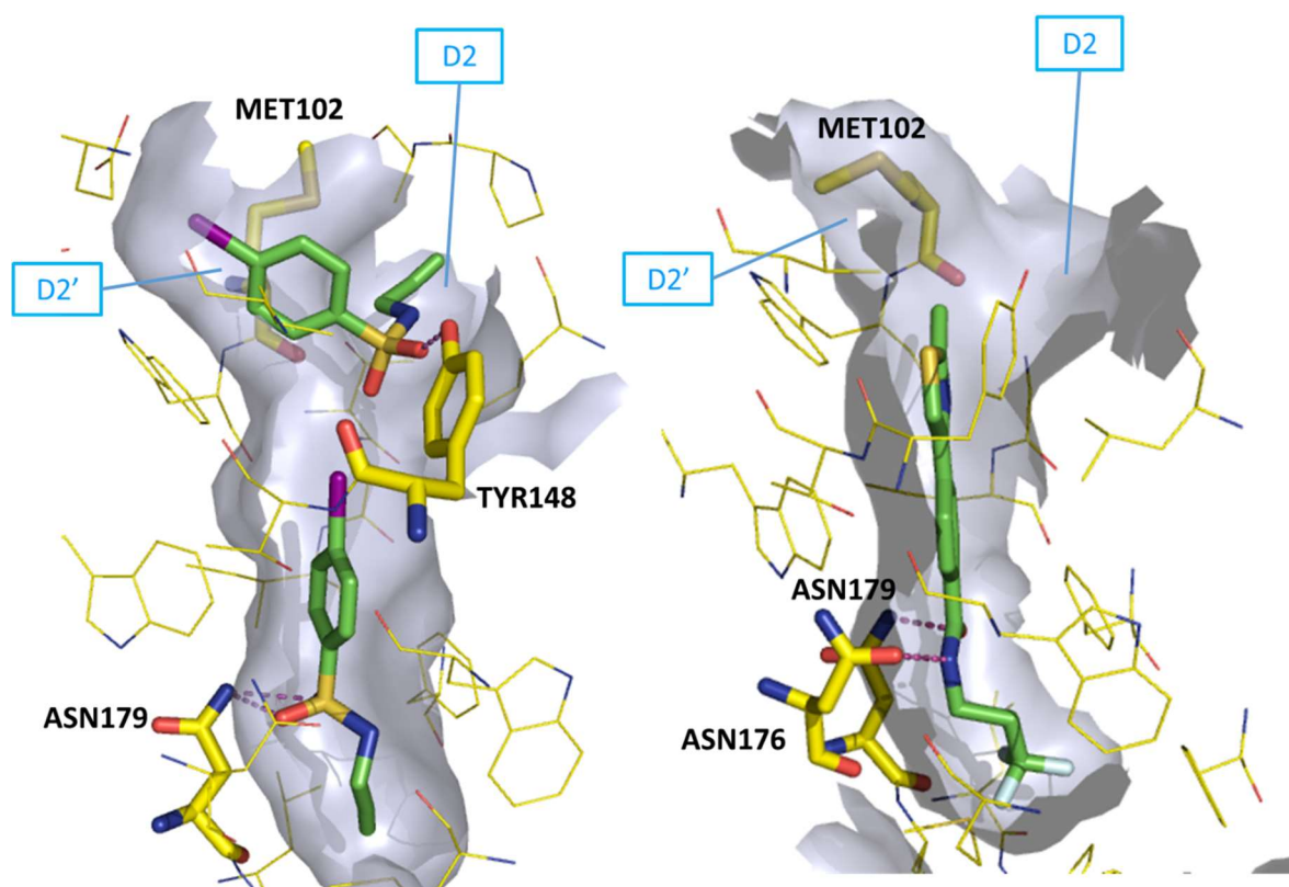
Figure 2. Binding mode of fragment 1 (left) and compound 3 (right, PDB ID 4M3B) to EthR.
