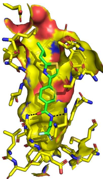
Figure 8. Binding mode of compound 13 to EthR.
