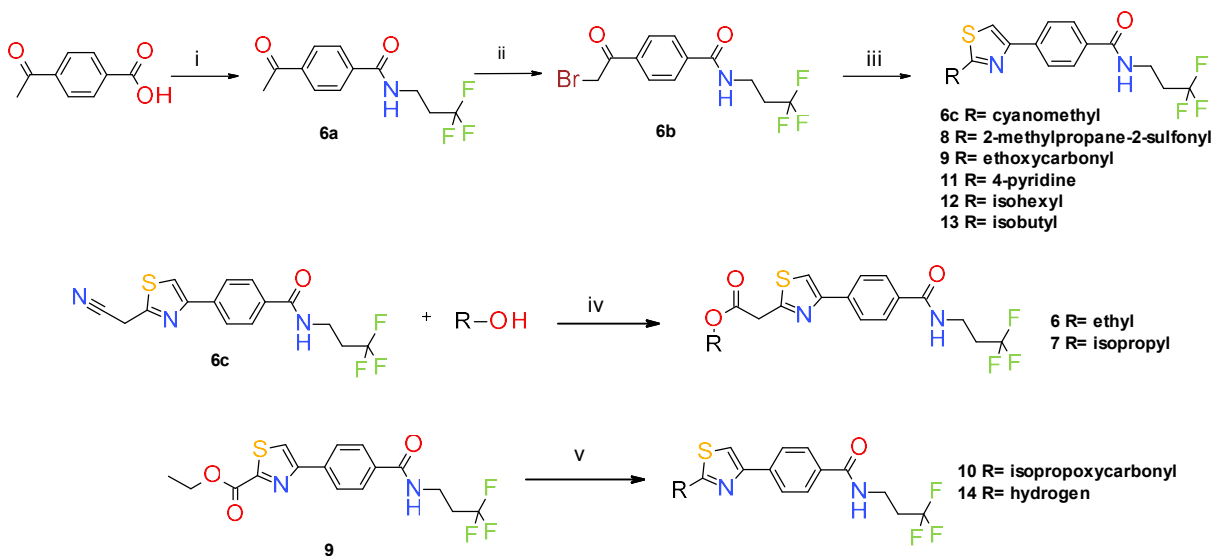
Figure 4. Synthesis of compounds 6-14. Reagents and reaction conditions : (i) 4-acetylbenzoic acid (1eq.), DIEA (4eq.), HBTU (1.2eq.), HOBT (0.2eq.), 3,3,3-trifluoropropylamine hydrochloride (1eq.), anhydrous DMF, RT, 2 h; (ii) trimethylphenylammonium tribromide (1.55eq.), DCE / MeOH (5/2), 50°C, 3 h; (iii) thioamide (1-1.4eq.), THF, reflux, 3-48 h; (iv)
