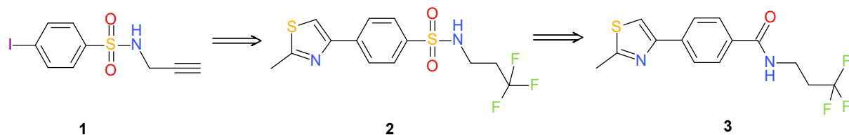
Figure 1. Structures of previously developed fragment-based EthR inhibitors 1, 2 and 3.
