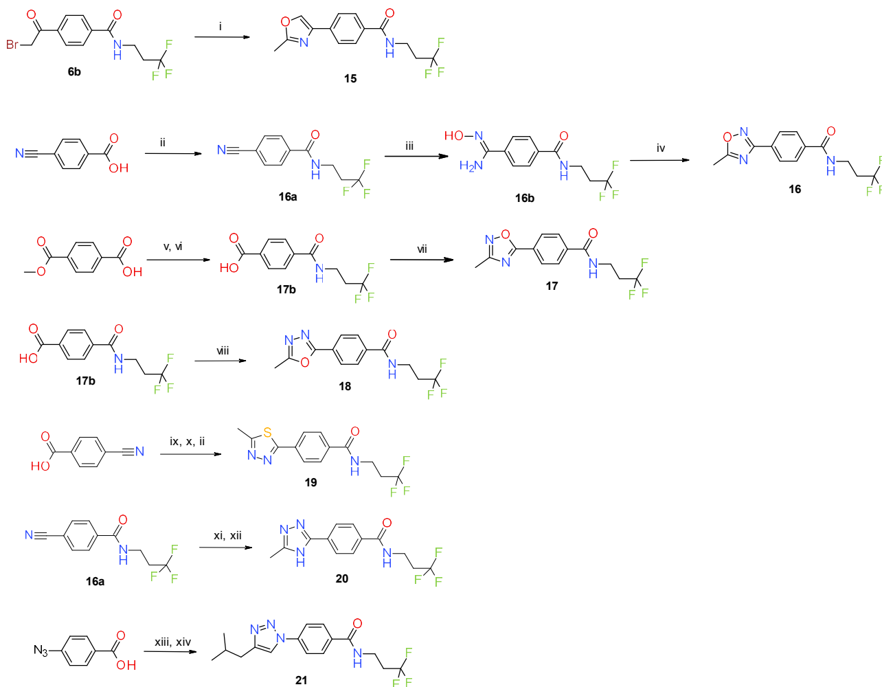
Figure 5. Synthesis of analogs 15 to 21. Reagents and reaction conditions: (i) Acetamide (1.2eq.), Toluene, 110°C, 10 min, \mu W irradiation; (ii) 3,3,3-trifluoropropylamine hydrochloride (1eq.), T3P® 50% w/w EtOAc (1.2-1.7eq.), DIEA (3-4eq.), EtOAc, RT, overnight; (iii) Hydroxylamine hydrochloride (1.5eq.), DIEA (1.6eq.), EtOH, reflux, 2 h; (iv) Acetic acid (1.1eq.), T3P® 50% w/w EtOAc (3eq.), DIEA (3.5eq.), EtOAc, reflux, 60 h; (v) 3,3,3-trifluoropropylamine
