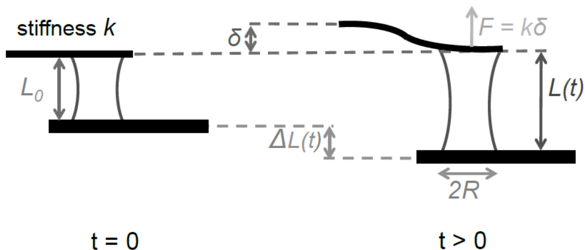
Figure 6: Principle of a creep experiment with the single cell rheometer. A cell is caught between two microplates, a flexible one (top, stiffness k ) and the rigid one (bottom, much stiffer than cells). At the beginning of the experiment, the flexible microplate is displaced by a distance \delta , held constant over time by a feedback loop applying a displacement \Delta L(t) = L(t) - L_0 to the rigid microplate. The constant applied stress is calculated from the displacement \delta , while the cell strain is retrieved from its elongation \Delta L(t) .
