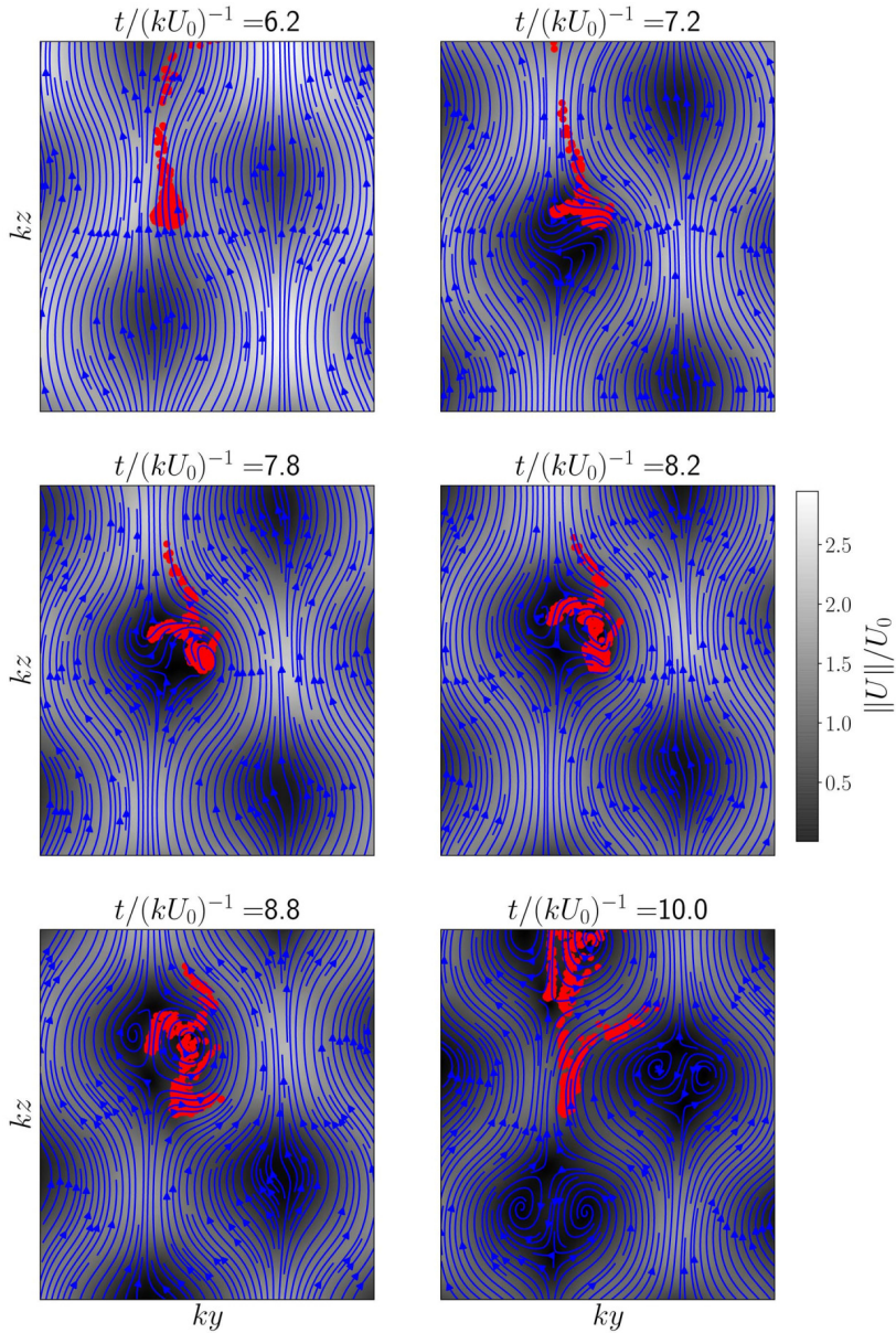
FIGURE 11. Flow field computed at successive times in the vertical plane in the cloud reference frame for a typical Oseenlet simulation in case C2b . High (low) velocity is indicated in white (dark). The corresponding movie 6 is available in the supplementary material.
