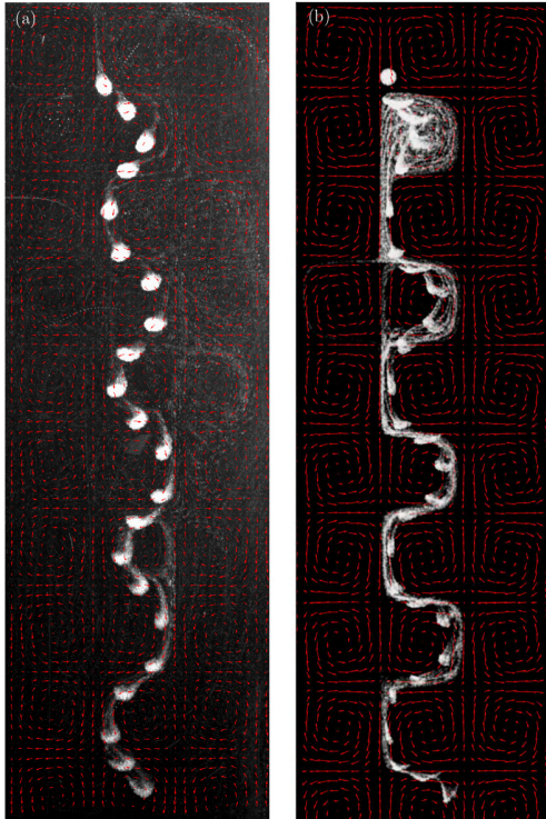
FIGURE 5. Same as figure 4 but for case B1b . The complete dynamics for the experimental case and for the Stokeslet simulation are shown in supplementary movie 2.
