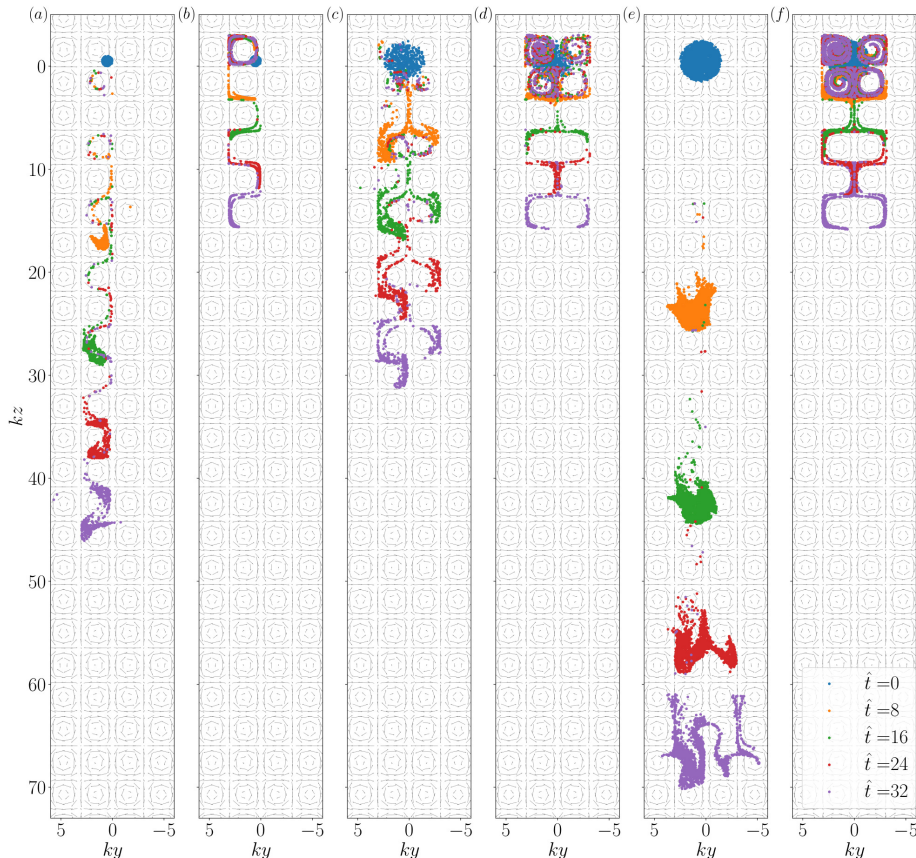
FIGURE 12. Snapshots of numerical clouds (using the Oseenlet approximation) corresponding to case C2a ( P = 0.03 , W = 0.108 , \ell/R_c = 2 ) settling in Taylor-Green vortices at five different times \hat{t} = t/(kU_0)^{-1} = 0, 8, 16, 24, 32 (each time \hat{t} corresponds to a different colour) with (a) Q = 0.5 and N_0 = 500 , (c) Q = 2 and N_0 = 500 , and (e) Q = 2 and N_0 = 2000 . Conditions in (b), (d), (f) are the same as in (a), (c), (e), respectively, but hydrodynamic interactions between particles have been switched off. The corresponding movie 7 is available in the supplementary material.
