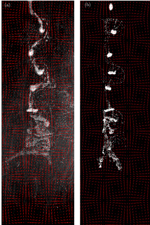
FIGURE 6. Same as figure 4 but for case C2b . The numerical simulation uses an Oseenlet (instead of Stokeslet) approximation. The complete dynamics for the experimental case and for the Oseenlet simulation are shown in supplementary movie 3.
