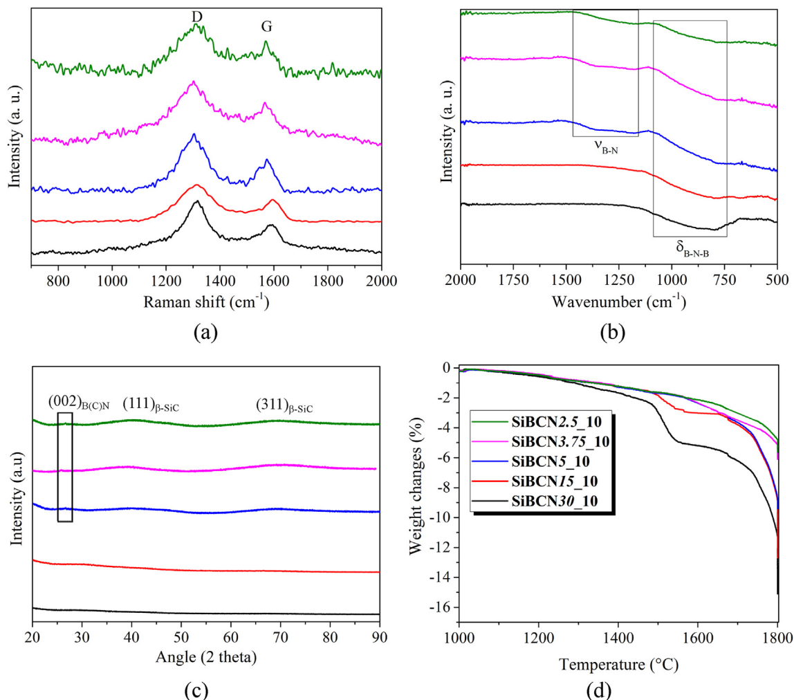
Fig. 2. Raman (a) and FTIR (b) spectra, XRD patterns (c) and TG curves (d) of as-pyrolysed samples with selected Si:B ratios.
