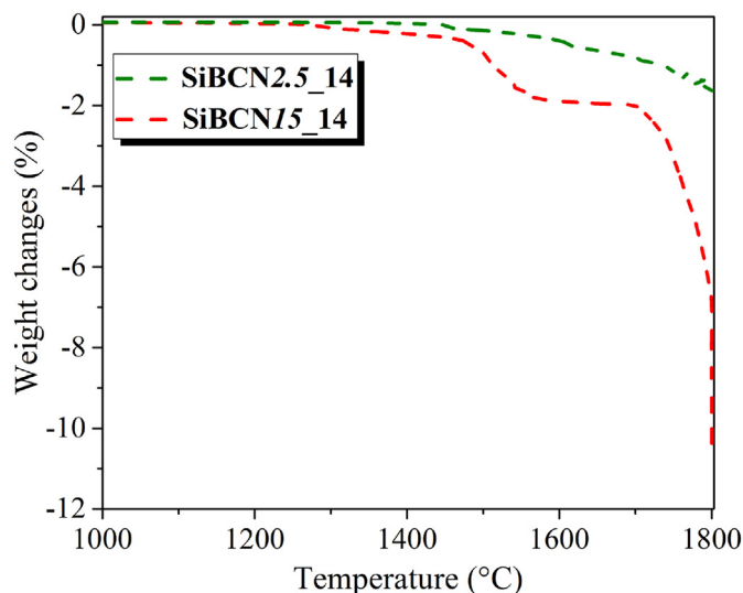
Fig. 3. TG curves of the SiBCN15_14 and SiBCN2.5_14 samples.
