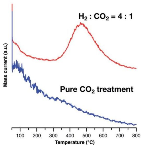
Fig. 9 Post reaction TPD-MS profiles of CO_2 ( m/z 44) under an Ar flow. The measurements were performed after exposure to a mixed gas with a 4 : 1 molar ratio of H_2 and CO_2 (Red) and pure CO_2 at 400\text{ }^\circ\text{C} (Blue).
