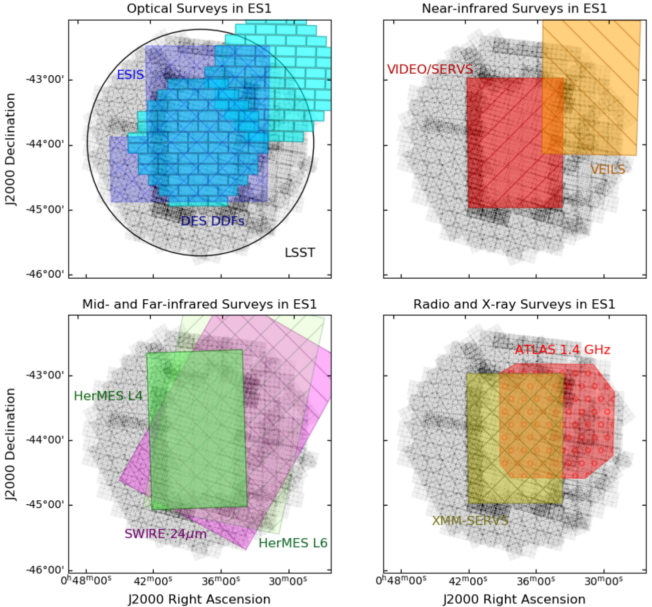
Figure 2. The footprints of multiwavelength surveys on the ELAIS-S1 field (see Table 2 for survey references), superimposed on a greyscale of the IRAC 4.5 \mu\text{m} coverage. Upper left: optical surveys (the DES DDFs are shown in cyan with rectangles indicating the individual chips, the ESIS survey in mauve with cross-hatches, and the LSST footprint is shown as a black circle); upper right, near-infrared surveys (VIDEO in red, left hatched and VEILS in orange, right-hatched). Lower left, 24 \mu\text{m} coverage from SWIRE in magenta and far-infrared coverage in HerMES in green (the L4 data are deeper than the hatched L6 data); lower right: the X-ray XMM -SERVS coverage in yellow, cross-hatched and the ATLAS radio survey in red, with circular hatches.
