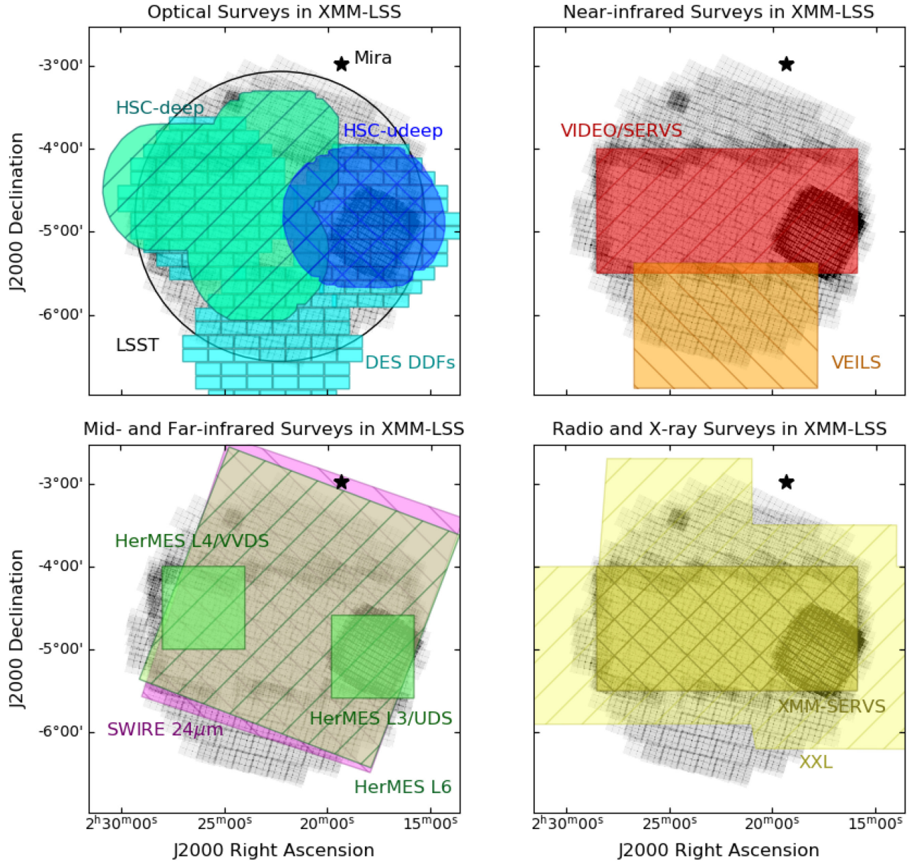
Figure 3. The footprints of multiwavelength surveys on the XMM-LSS field (see Table 2 for survey references), superimposed on a greyscale of the IRAC 4.5 \mu\text{m} coverage. Upper left: optical surveys (the LSST footprint is shown as a black circle, the DES DDFs are in cyan with rectangles indicating the individual chips, the HSC-deep survey is in green with left hatches, the HSC-ultradeep in blue with cross-hatching). Upper right: near-infrared surveys (VIDEO in red, left hatched and VEILS in orange, right-hatched). Lower left: 24 \mu\text{m} coverage from SWIRE in magenta and far-infrared coverage from HerMES in green (the L3 data are the deepest, L4 less deep and L6 the shallowest). Bottom right: X-ray surveys – the XXL survey coverage is shown in light yellow, left-hatched and the XMM-SERVS survey in dark yellow, cross-hatched). The position of the infrared-bright, variable star Mira ( K \approx -2.2 ) is indicated with the black star symbol.
