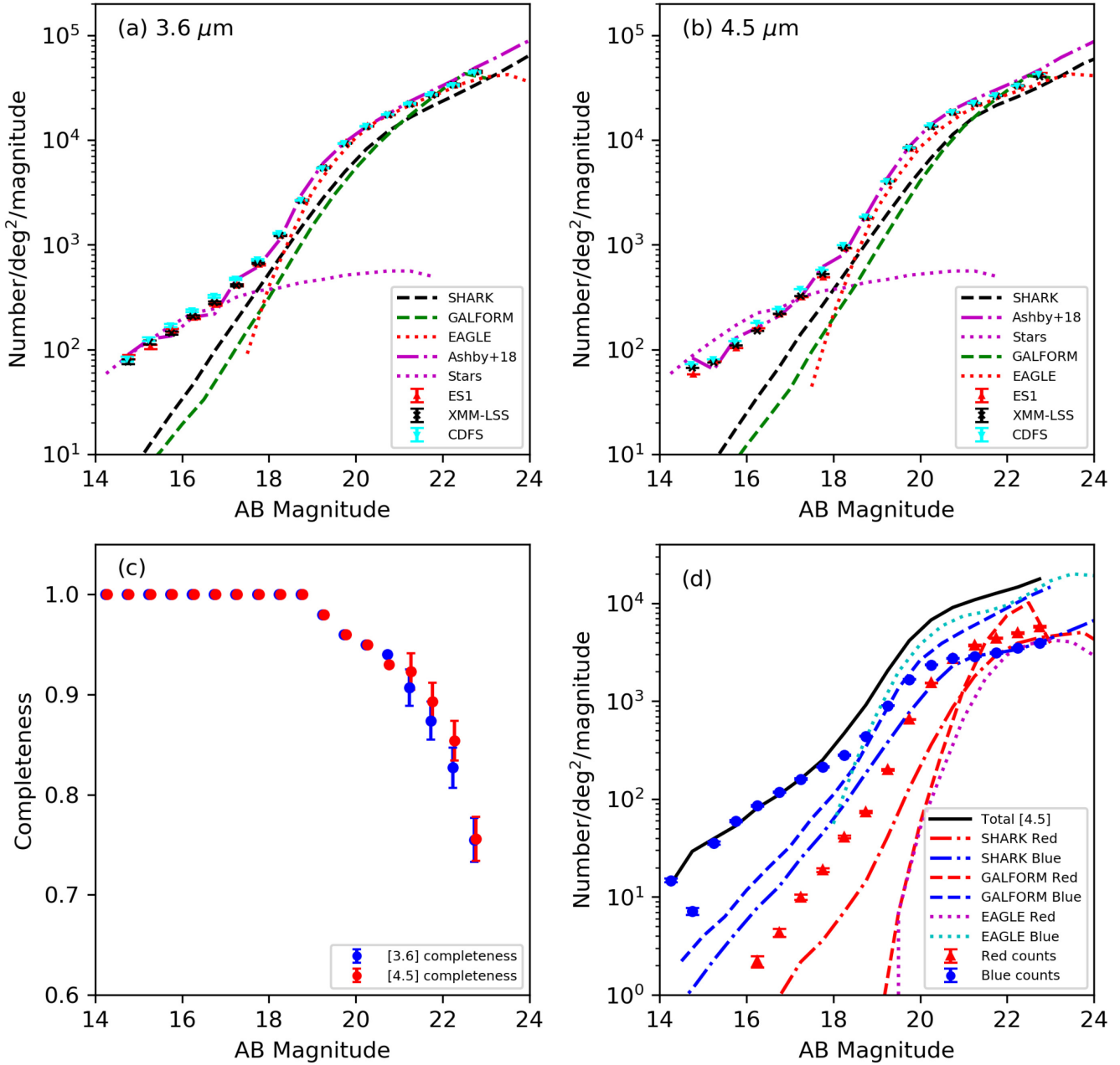
Figure 8. DeepDrill source counts. (a) The 3.6 \mu\text{m} counts: the three sets of points show the completeness-corrected counts from each DeepDrill field. The dot-dashed magenta line shows the mean counts from the S-CANDELS fields (Ashby et al. 2015). The magenta dotted line shows star counts from the UDS field (which is within the DeepDrill XMM-LSS field) from Ashby et al. (2015), using the model from Wainscoat et al. (1992) as refined by Cohen (1993), Cohen (1994), Cohen (1995), and Arendt et al. (1998). (As all three fields have Galactic latitudes of -60^\circ \pm 15^\circ these will be representative of the survey as a whole.) The dashed black and green lines show the galaxy counts from the SHARK (Lagos et al. 2018, 2019) and GALFORM semi-analytic simulations, respectively, and the dotted red line those from the EAGLE hydrodynamic simulations. (b) The same for the 4.5 \mu\text{m} counts. (c) The survey completeness as a function of magnitude. (d) Counts for red ( [3.6] - [4.5] > 0.1 ) and blue ( [3.6] - [4.5] < -0.3 ) sources separately, with the total [4.5] counts also shown, along with model counts from SHARK, GALFORM and EAGLE.
