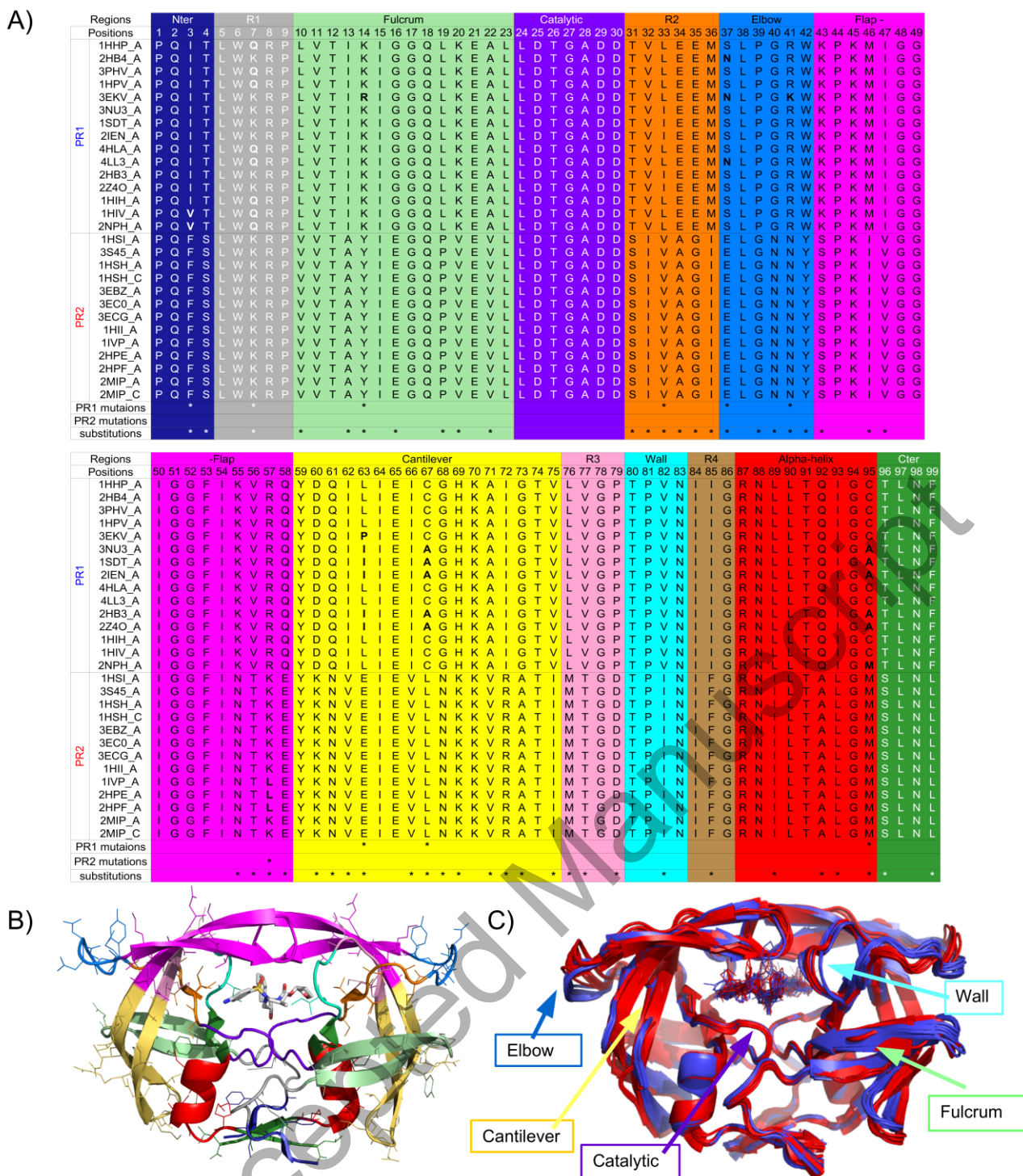
FIGURE 1. Presentation of the PR1 and PR2 structure sets. A) Multiple alignment of 24 PR1 and PR2 sequences. The alignment is coloured according to the 13 extracted PR regions. B) Visualization of the three-dimensional structure of PR2 complexed with APV (PDB code: 3S45). The PR2 structure is displayed in cartoon mode and coloured according to the 13 extracted PR regions. Substituted residues between PR1 and PR2 are displayed as sticks. The colour code for
