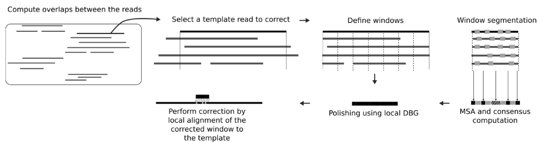
Figure 1. Overview of CONSENT's workflow for long read error correction.
