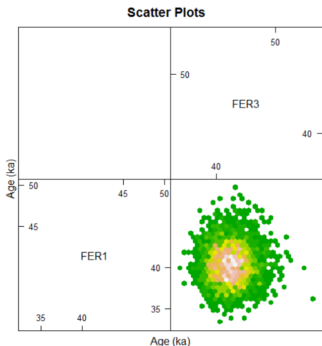
Figure 2. Bivariate scatter plot as hexagon plot presentation of a sample of observations from the joint posterior distribution of the two OSL ages considered independently (no stratigraphic constraints, no off-diagonal members in the covariance matrix). In such a plot, each point corresponds to one realisation of the ages of the two samples generated by the MCMC. Note that the reason for having this figure in the cell of an array is not visible here; it becomes useful when calculating ages for more than two samples, in which case for each pair of samples, a similar plot appears in the appropriate cell.
