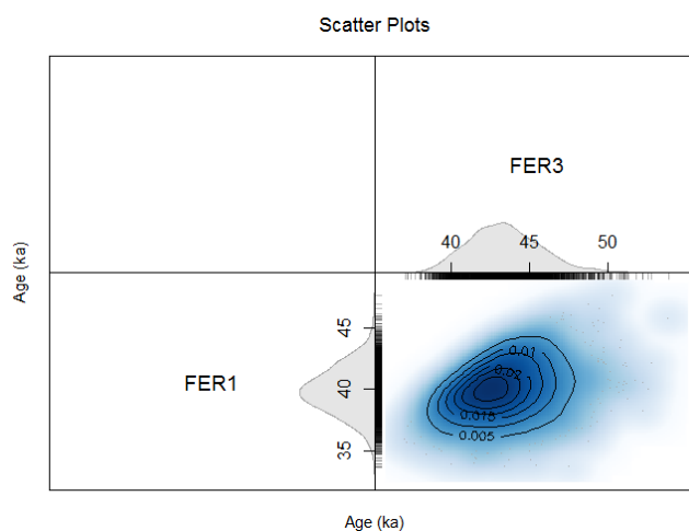
Figure 5. Probability densities for the OSL ages estimated jointly, using the same model as that implemented to generate Fig. 4 (stratigraphic constraint, no covariance matrix).
