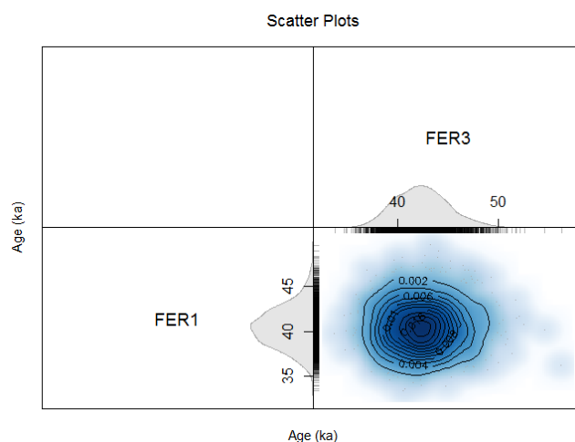
Figure 3. Probability densities for the OSL ages estimated jointly with the same model as that used to generate Fig. 2, based on kernel density estimates (KDEs), and marginal probability densities. The bell-shape and symmetry of the scatter plot indicate the absence of correlation between the two ages.
