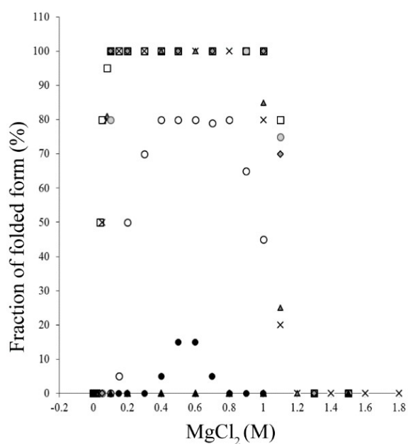
FIG.5. Salt-concentration dependent stability curves of various halobacterial MalDHs in MgCl_2 . Modern enzymes: H. mukohatei from group A (grey squares), H. volcanii from group B (open squares) and N. magadii from group C (black dots). Ancestral MalDHs: Anc78 (crosses), Anc80
