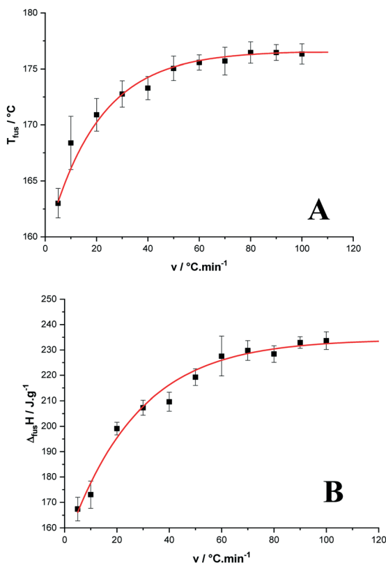
Fig. 6 Temperature (A) and enthalpy (B) of melting of p -syneprine enantiomers as functions of the heating rate.
