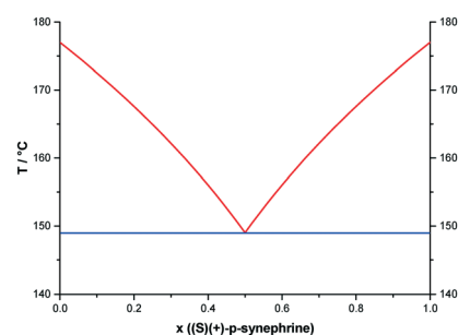
Fig. 8 Temperature-composition solid-liquid metastable phase diagram of the ( R )-/-( S )- p -syneprine binary system. The ideal liquidus curves (red lines) are obtained using the Schröder-van Laar equation.
