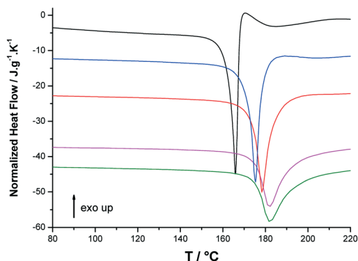
Fig. 5 Selected normalized DSC curves of (R)-(-)- p -syneprine at 5 (black), 20 (blue), 40 (red), 80 (magenta) and 100 °C min -1 (green).
