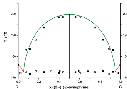
Fig. 7 Temperature-composition solid-liquid stable phase diagram of the R -/ S - p -syneprine binary system. x stands for the (S)-(+)-enantiomer composition. The experimental data obtained from the thermograms are represented by solid squares and the ones obtained by symmetry are represented by empty squares. Prigogine-Defay and Schröder-van Laar ideal behaviors of the liquidus curves are represented in green and red lines, respectively. The blue line corresponds to the mean value of the eutectic invariant obtained from DSC experiments.
