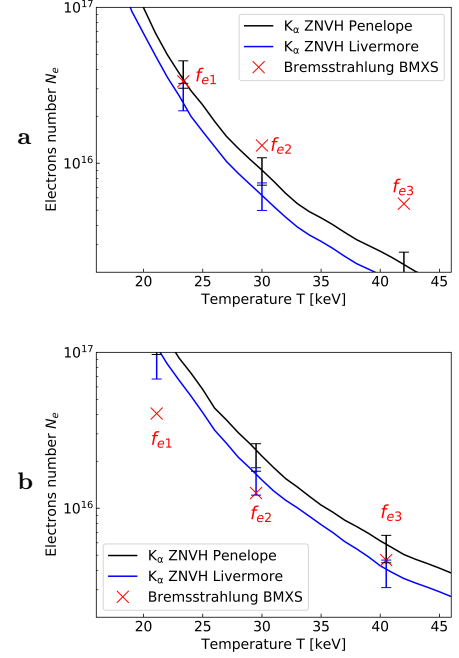
FIG. 11: Map of possible values of N_e and T_h that can reproduce the experimental data ( K_\alpha and bremsstrahlung spectrum) for shots #28406 (a) and #28407 (b). The black and the blue lines result from K_\alpha simulations with libraries Penelope and Livermore, respectively. The red crosses indicate the average values coming from the two BMXS, using the three representative points scheme. The experimental error on the K_\alpha signal, evaluated to be around 20%, is shown by error-bars.
