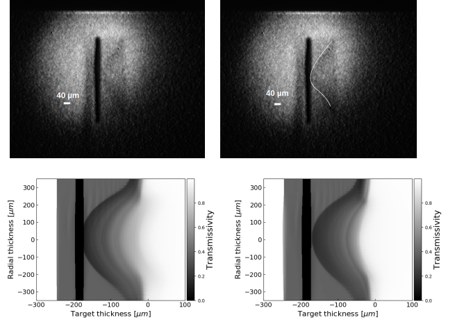
FIG. 19: [Top] Experimental radiography of shot #28407 at 1.650 ns. In [Top-Right] the shock front is highlighted; [Bottom-left] synthetic radiography obtained by the simulation with f_{e1}(E) at t = 1.700 \text{ ns} ; [Bottom-right] synthetic radiography obtained by the simulation with f_{e2}(E) at t = 1.700 \text{ ns} .
