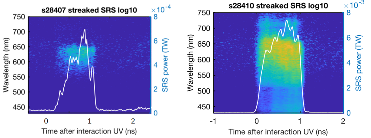
FIG. 16: Reflected light due to SRS and TPD collected by the SABS for shot #28407 and #28410. The bandwidth of the diagnostic ranges from 400 nm up to 750 nm. The temporal profile of the signal is indicated by the white line. The values of the SRS power collected are not significative, since the diagnostic covers only the 6% of the beam solid angle.
