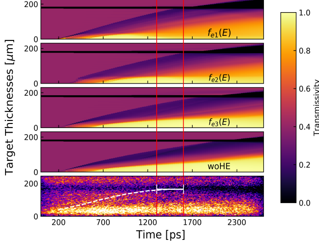
FIG. 21: Comparison between the experimental 1D time resolved radiography of shot #28412 and the synthetic ones. The three hot-electron cases (denoted f_{e_i} ) and the without HE (woHE) case are reported. The time at which the shock arrives on the plate is marked with red lines. The white dashed line indicates the progression of the shock.
