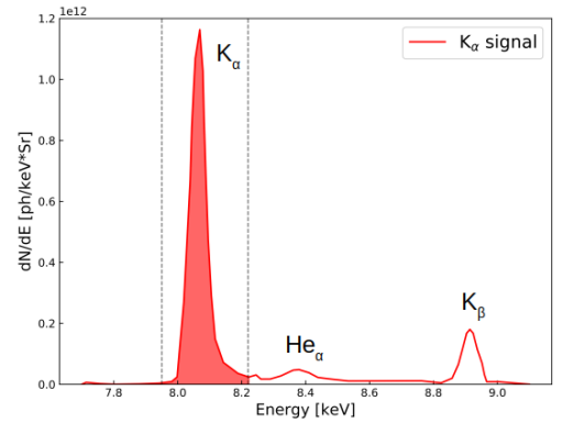
FIG. 6: X-ray spectrum detected by the ZNVH spectrometer for the shot #28407, after the background correction.
