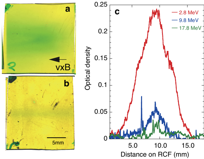
FIG. 4. a & b . 2nd and 10th RCF layer (corresponding to 2.8 and 9.8 MeV protons) images taken at 5 mg/cc foam target. The pulse duration and intensity in this shot were 300 fs and 2.5 \times 10^{19} W/cm 2 . The ions bent by the magnet come from right to left in this image. c . The vertical line profiles of each layer for 2.8, 9.8, and 17.8 MeV protons, respectively. Beam divergence calculated from the signal width are 12.7, 8.2 and 2.7° (FWHM).
