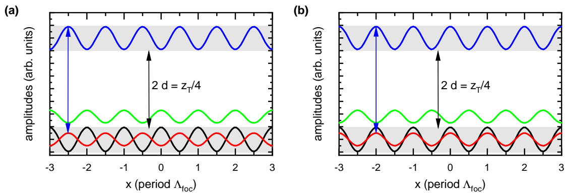
Figure 6. Illustration of feedback loop for single-mirror feedback for optomechanical interactions (see caption of Figure 2 for general explanation). Black line in atomic cloud denotes atomic density. (a) Blue detuning ( \Delta > 0 ): Atoms are low field seekers and hence atomic and intensity structures are complementary (atomic troughs align with intensity peaks, situation of experiment described in [44]). (b) Red detuning ( \Delta < 0 ): Atoms are high field seekers and hence atomic and intensity structures are aligned. Note that the nonlinearity is self-focusing also for red and blue detuning and the instability exists for both signs of the detuning (similar to [75] for the case of single-pass propagation).
