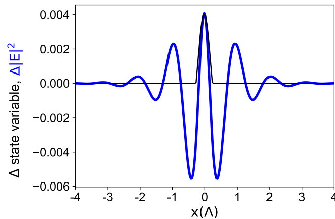
Figure 17. Perturbation of atomic state variable (black line) proportional to refractive index and resulting perturbation (scaled to meet perturbation amplitude for purpose of visualization) in intra-cavity intensity after a time corresponding to five times the inverse of the cavity decay rate (see text and Figure 15 for details of the procedure). Parameters: pump intensity 1.05 above threshold; cavity detuning zero, \Delta = -10\Gamma , cooperativity parameter C = 0.0125 .
