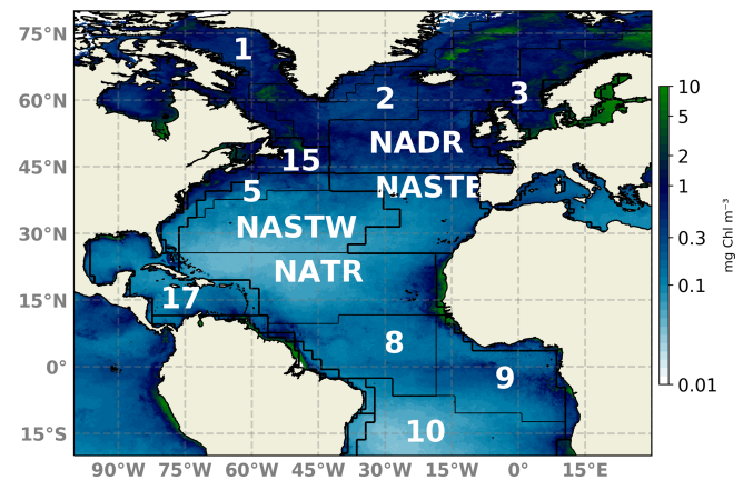
Figure 1. Schematic map of the North Atlantic basin showing the NATL-025/PISCES domain. Longhurst et al. (1995) biogeochemical provinces are indicated. Provinces are indicated by abbreviations: NADR (North Atlantic Drift), NATR (North Atlantic tropical gyre), NASTE (northeast Atlantic subtropical gyre), and NASTW (northwest Atlantic subtropical gyre) are used throughout the text. A 2018 yearly composite of sea surface Chl a is superimposed.
