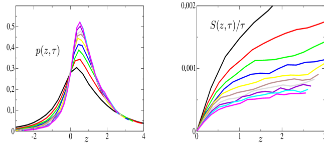
Figure 2. The pdf p(z, \tau) (left) and the symmetry function normalised by the averaging time S(z, \tau)/\tau (right) as a function of z for different averaging times \tau (see caption and legend of Fig. 1); data are from GSE, res 0.5^\circ , 1993–2016, res 6h
