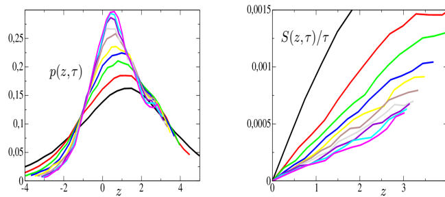
Figure 3. The pdf p(z, \tau) (left) and the symmetry function normalised by the averaging time S(z, \tau)/\tau (right) as a function of z for different averaging times \tau (see caption and legend of Fig. 1); data are for case PSG, res 0.5^\circ , 1993–2016, res 6h
