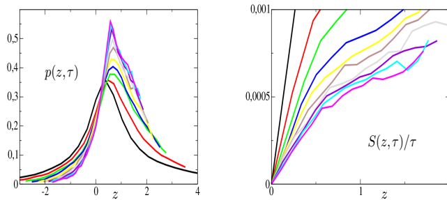
Figure 4. The pdf p(z, \tau) (left) and the symmetry function normalised by the averaging time S(z, \tau)/\tau (right) as a function of z for different averaging times \tau (see caption and legend of Fig. 1); data are for case KUE, res 0.5^\circ , 1993–2016, res 6h
