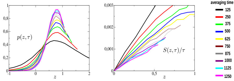
Figure 1. The pdf p(z, \tau) (left) and the symmetry function normalised by the averaging time S(z, \tau)/\tau (right) as a function of z for different \tau (see caption). The variable \tau gives the length of the averaging interval in terms of observations done every 6 hours. Data are for case ASG, res 0.5^\circ , 1993–2016, res 6h
