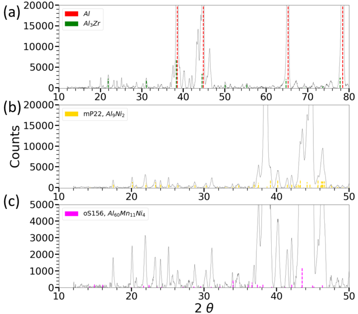
Figure 5: XRD patterns obtained from an as-built sample. (a) In the (10°, 80°) angular range, the main diffraction peaks are indexed as FCC-Aluminium ( a=4.04317 \text{ \AA} , red dashed lines) and \text{Al}_3\text{Zr-L1}_2 structure ( a=4.069 \text{ \AA} , green dashed lines). (b) and (c) Enlarged views of the XRD patterns in the 10-50° range. (b) The yellow dotted lines can be indexed as a monoclinic structure with lattice parameters a = 6.23752 \text{ \AA} , b=6.28521 \text{ \AA} , c=8.62636 \text{ \AA} , \beta=95.705 consistent with the \text{Al}_9\text{Ni}_2 phase (structure type \text{Al}_9\text{Co}_2 , Pearson symbol mP22). (c) The pink dotted lines can be indexed as an orthorhombic structure with lattice parameters a = 7.55 \text{ \AA} , b=23.8 \text{ \AA} , c=12.5 \text{ \AA} associated to the structure type \text{Al}_{60}\text{Mn}_{11}\text{Ni}_4 phase (Pearson symbol oS156). The XRD indexing is based on the crystallographic information from the ICDD PDF4+ database. Though the exact composition might be different, the various phases will be referred to by the chemical formula from this XRD database.
