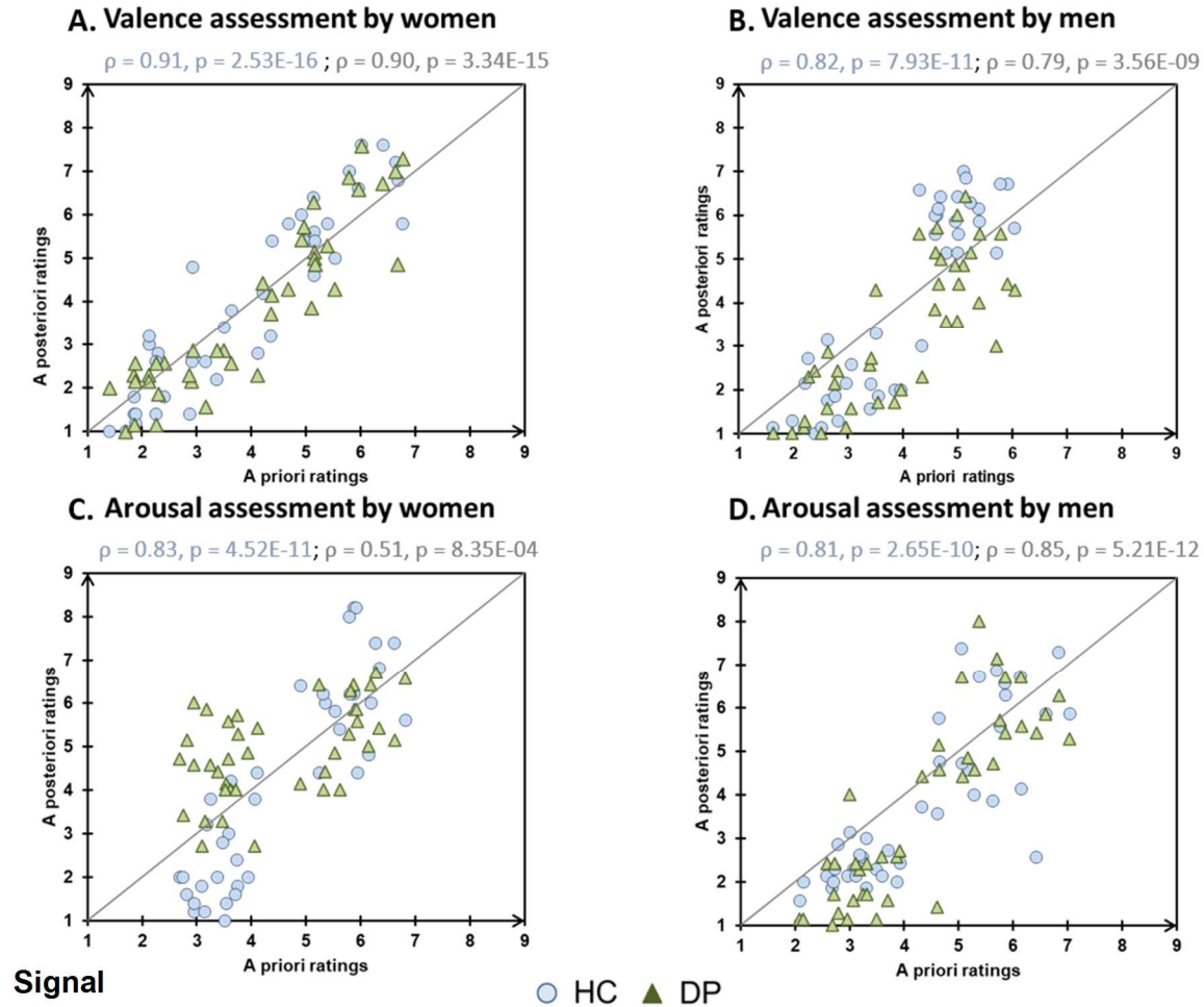
Figure 1. Validation of picture selection using correlations between standardised ( a priori ) ratings according to the International Affective Picture System (IAPS) and mean subjective ( a posteriori ) ratings of unpleasant and neutral pictures. Ratings for controls (HC) are represented in blue and ratings for patients (DP) in green. (A) Valence ratings for women; (B) valence ratings for men; (C) arousal ratings for women; (D) arousal ratings for men. A posteriori ratings did not depend on group or gender (All F_s < 3.11 and p_s > 0.091 ).
