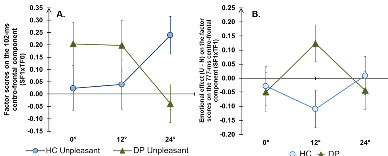
Fig. 5. Eccentricity effect on 102 ms centro-frontal component (SF1xTF6) and for 777 ms centro-frontal component (SF1xTF1). (A) Data are estimated marginal means of 102 ms centro-frontal (SF1xTF6) factor scores for unpleasant pictures and (B) emotional effect (U – N) on 777 ms centro-frontal (SF1xTF1) factor scores with standard errors, according to position of stimuli (central: 0°; near periphery: 12° and far periphery: 24°), for healthy controls (HC, blue lines) and depressed patients (DP, green).
