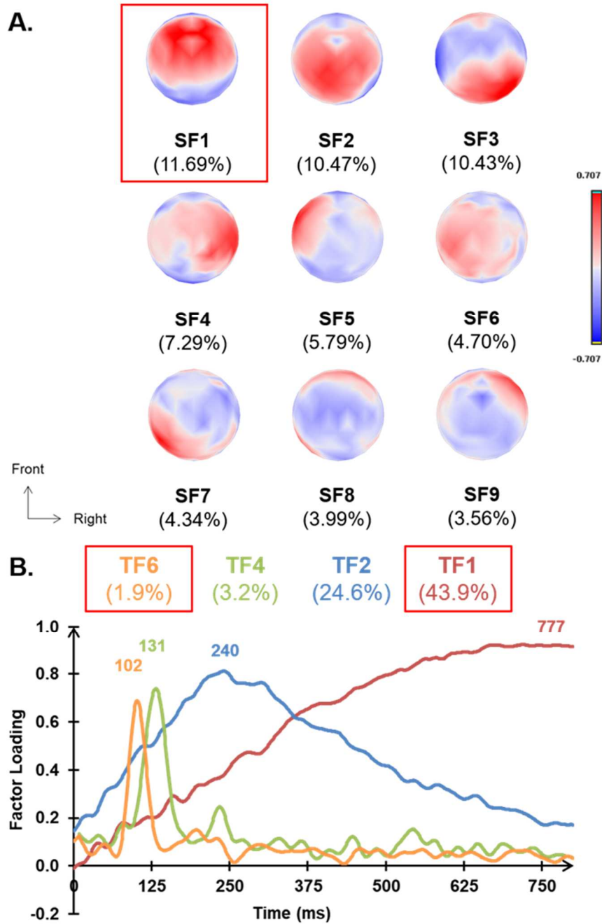
Fig. 4. Topographic map of factor loading for selected spatial factors (SF) from combined spatial principal component analysis (sPCA) and temporal principal component analysis (tPCA) solution for SF1 component. (A) Superior view of topographic map of factor loading for selected SF with percentage of variance accounted for by each SF. (B) Time at peak and percentage of variance accounted for by each temporal factor for SF1 component.
